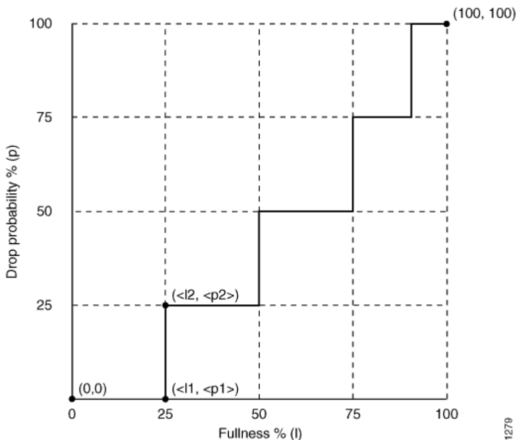
Figure 3: Graphical Representation of a Segmented Drop Profile
