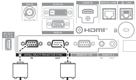
Connecting terminals of the first projector
