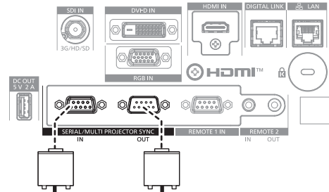
Connecting terminals of the second projector
