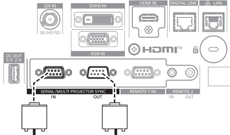
Connecting terminals of the fourth projector
