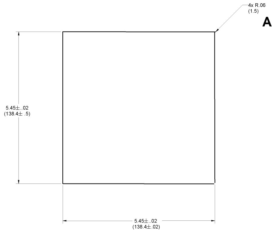
Figure 3-4: Panel Cut-out
