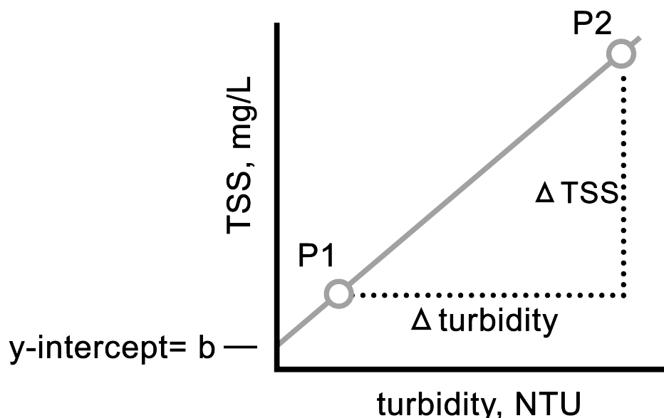
Figure 7-6: Converting Turbidity to TSS
