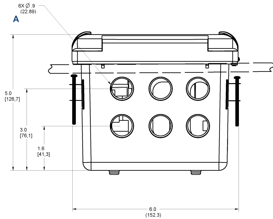
Figure 3-3: Panel Mount Bottom View
