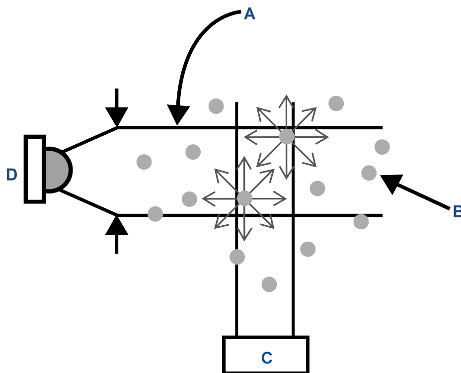
Figure 7-5: Turbidity Sensor - ISO 7027
