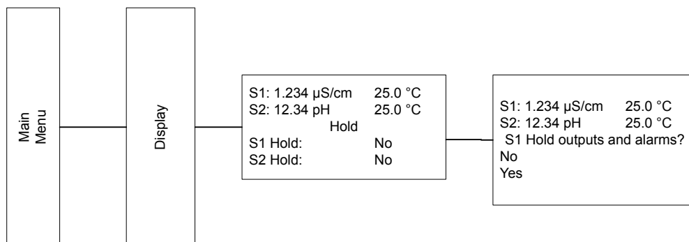
Figure 6-3: Using Hold
