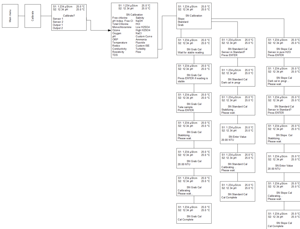
Figure 8-1: Calibrate Turbidity
