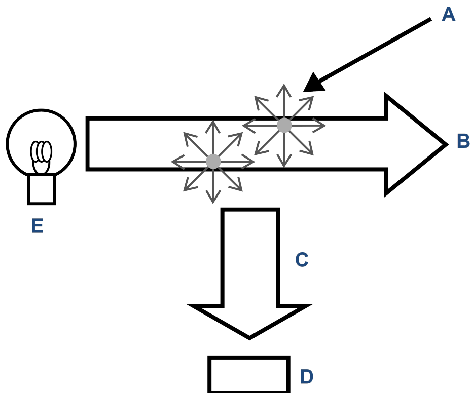
Figure 7-3: Turbidity Sensor - General
