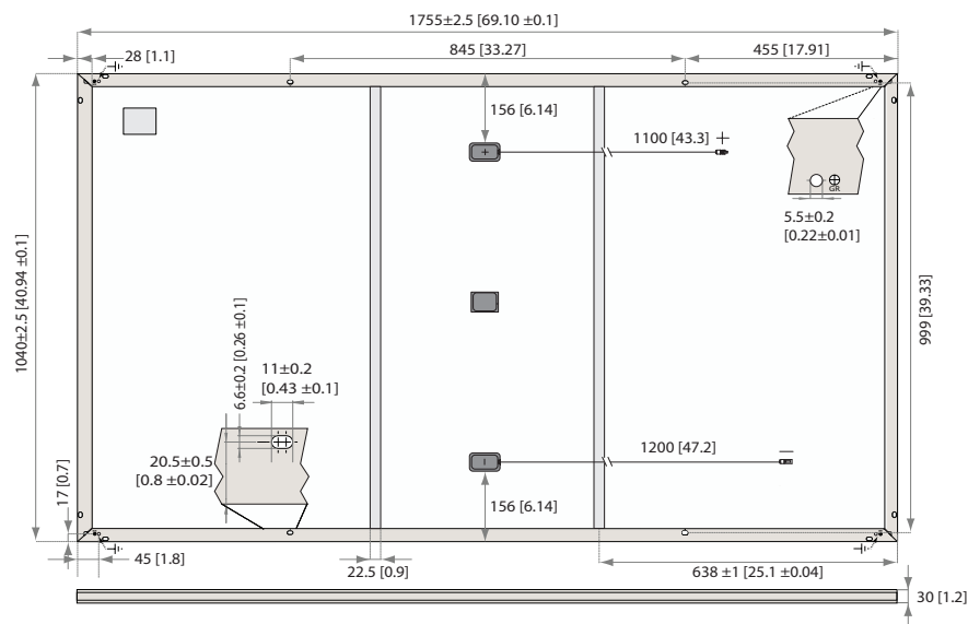
Fig. 24: Panel dimensions: REC N-Peak 2 Series
