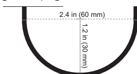
Fig. 19: Minimum cable bend radius
