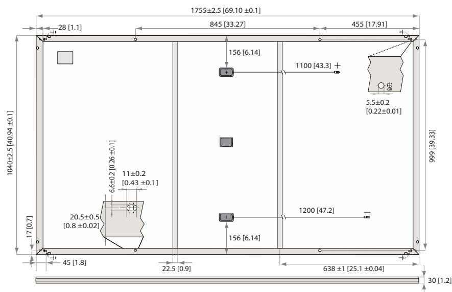
Fig. 25: Panel dimensions: REC N-Peak 2 Black Series
