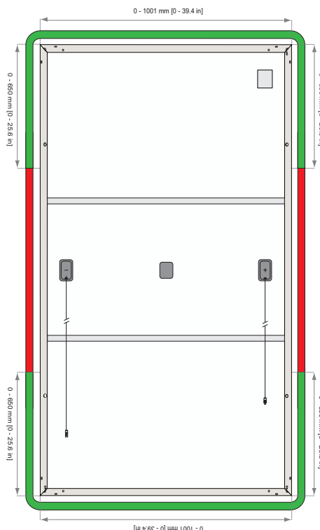
Fig. 27: REC 72-cell panels MLPE device installation zones
