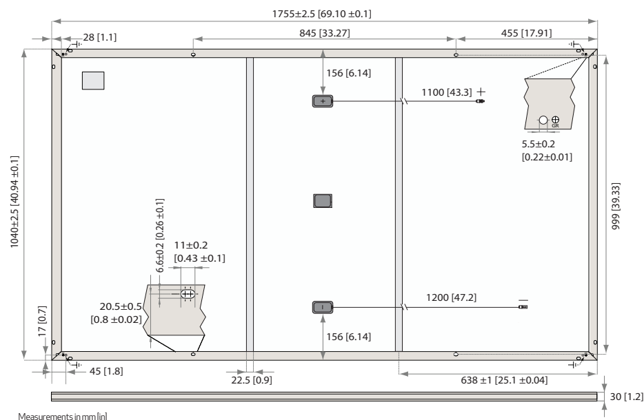
Fig. 21: Panel dimensions: REC TwinPeak4 Black Series
