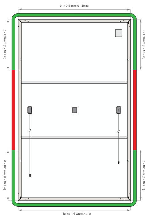
Fig. 26: REC 60-cell panels MLPE device installation zones
