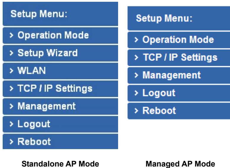
Figure 5-1 Main Menu
