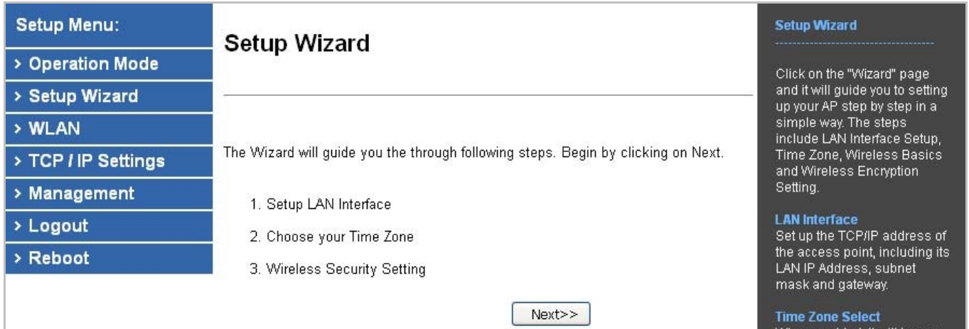
Figure 5-3 Setup Wizard
