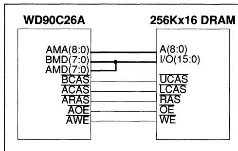
FIGURE 6-11 TYPICAL 256Kx16 DRAM INTERFACE
