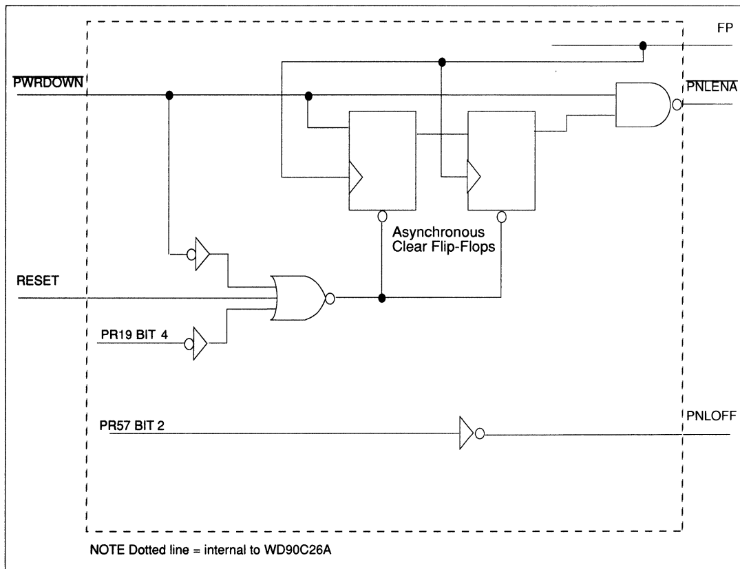
FIGURE 6-15 PNLENA AND PNLOFF PANEL PROTECTION SIGNALS
