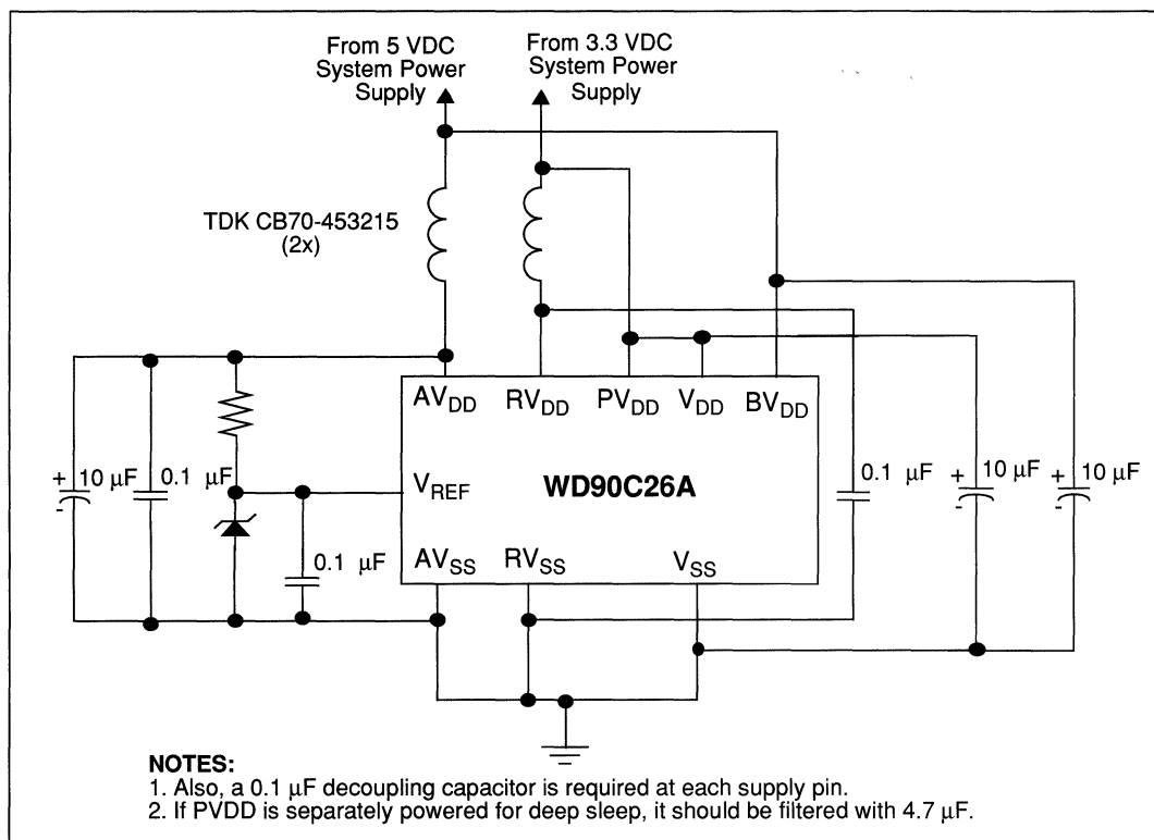
FIGURE 6-7 RECOMMENDED POWER SUPPLY ISOLATION AND DECOUPLING FOR MIXED VOLTAGE OPERATION
