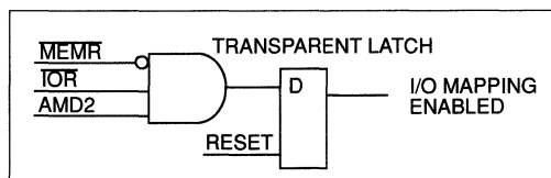
FIGURE 6-33 ENABLING I/O MAPPING ON THE WD90C26A
