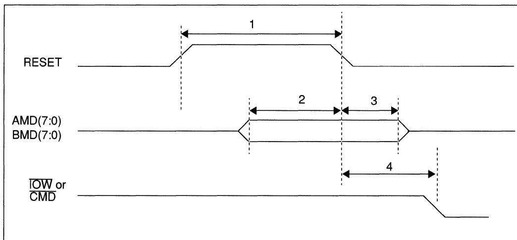
FIGURE 11-2 RESET TIMING
