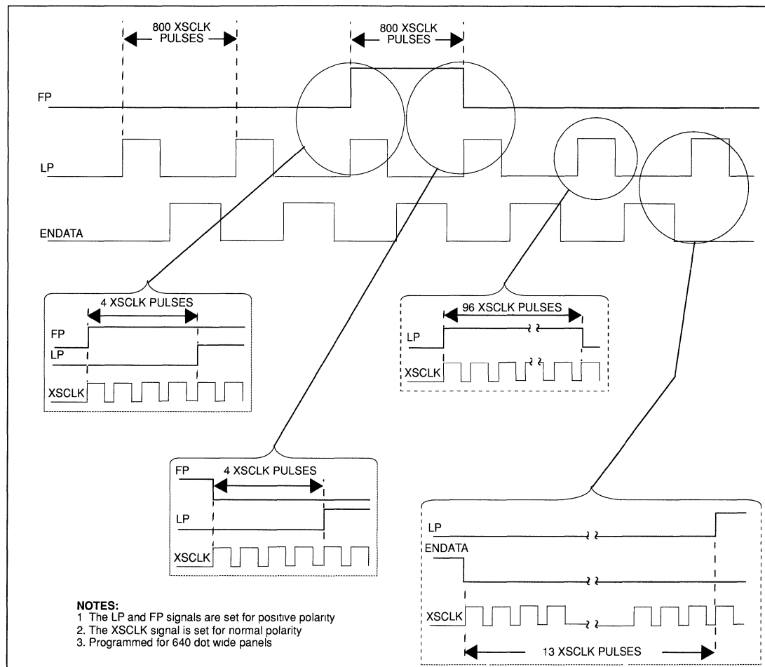
FIGURE 11-9 TFT PANEL FUNCTIONAL TIMING
