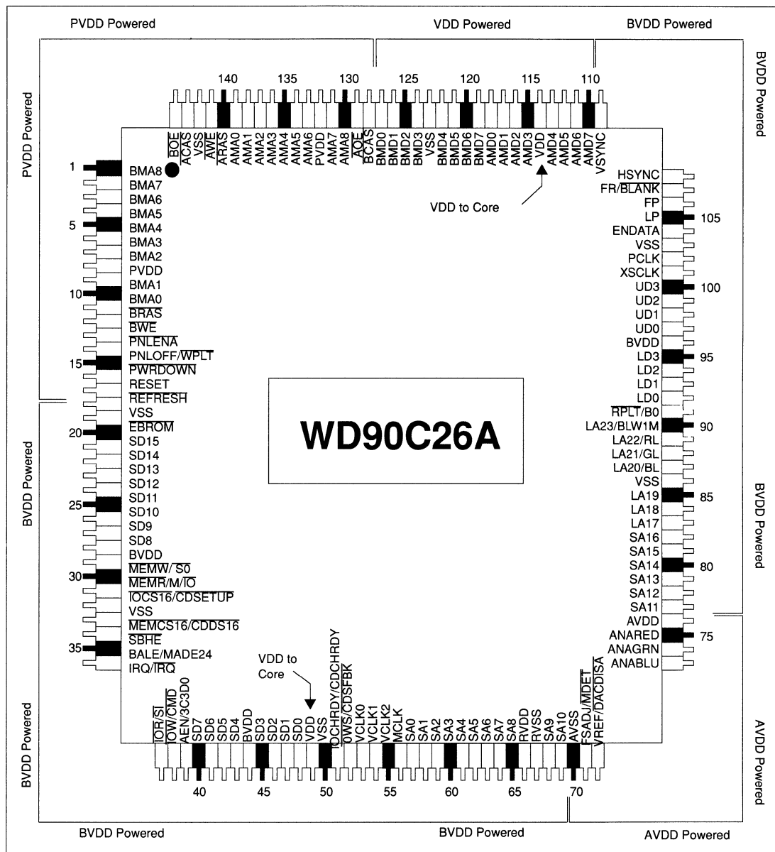
FIGURE 6-1 POWERING OF WD90C26A I/O PINS
