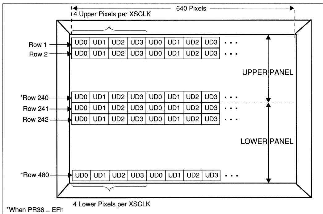
FIGURE 6-26 DUAL PANEL LCD DATA ORGANIZATION
