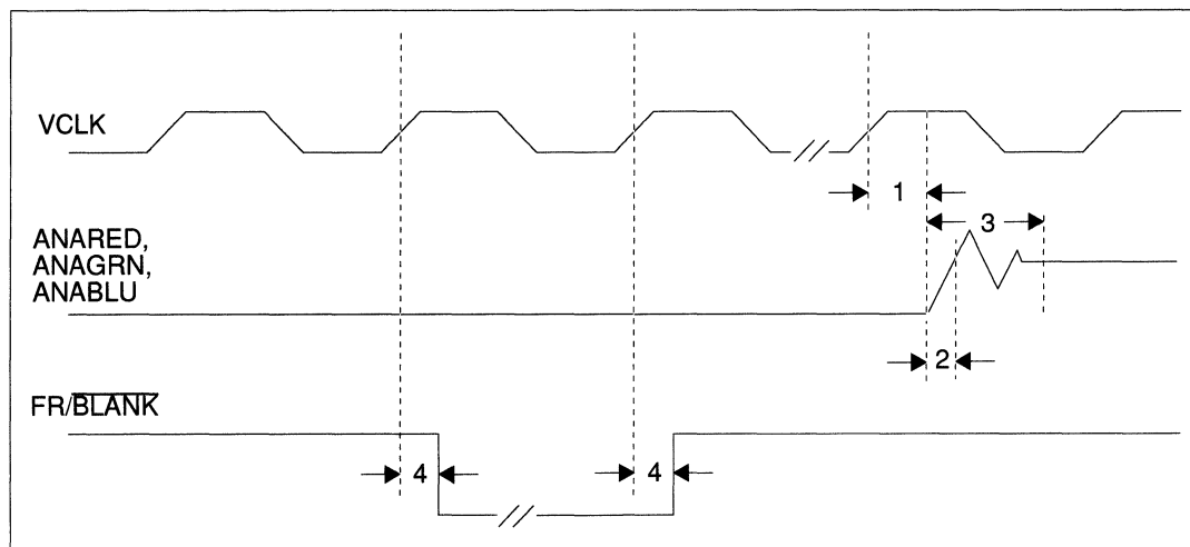
FIGURE 11-10 RAMDAC TIMING
