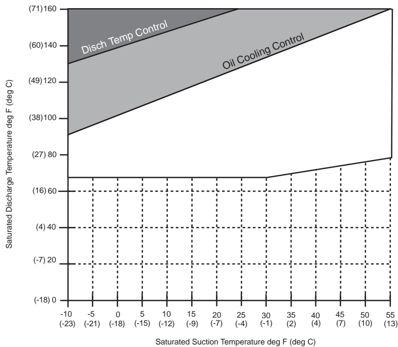
R-134a APPLICATIONS
