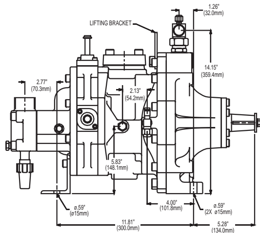
Dimensions (Top View)
