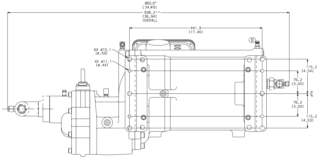
BOTTOM VIEW
