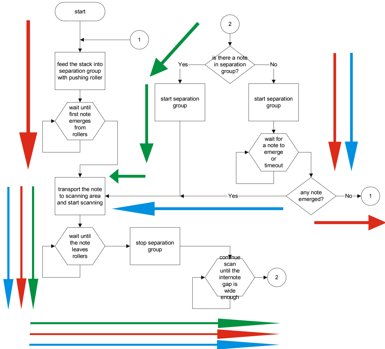
Fig. 26. Generalized stack processing
