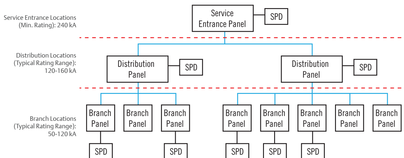
Figure 1: Cascaded Surge Suppression | IEEE Standard 1100
