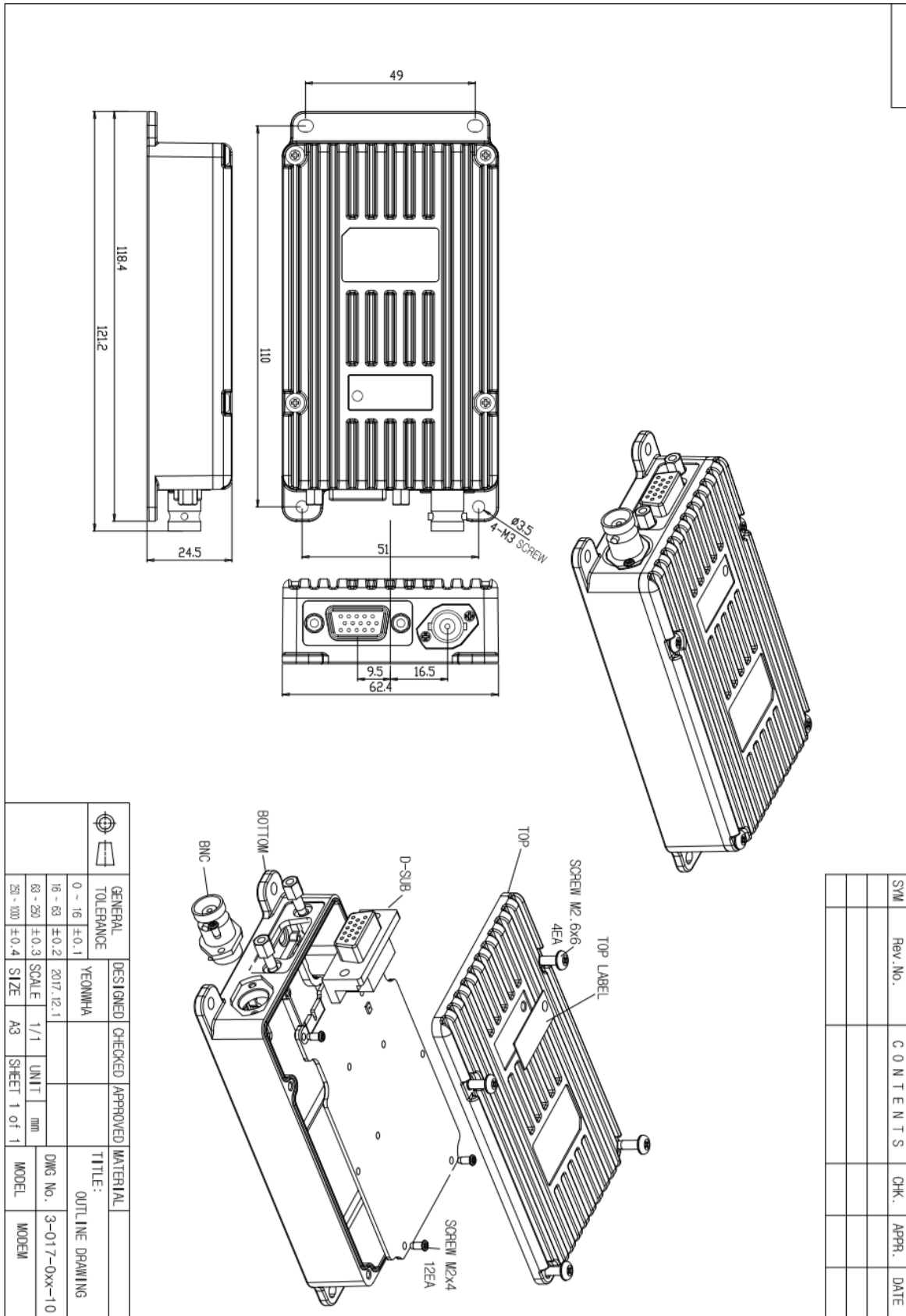
Figure 3-4) SD-671D/674D Drawing
