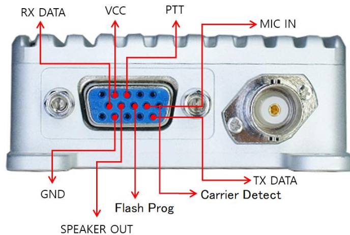
Picture 3-2) Main Pin Specification
