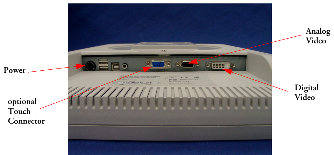
Figure 24 Connections M8033A
