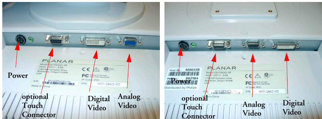
Figure 25 Connections M8033B (old and new version)
