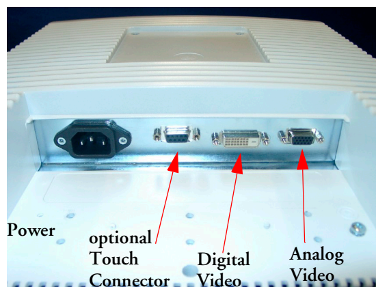
Figure 26 Connections M8033C
