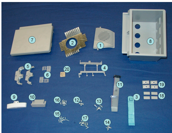
Small Parts Kit 1
