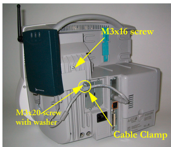
Proxim Wireless Ethernet Adapter
