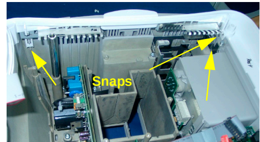
Bottom Edge of Housing
