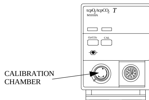
M1018A Traditional CMS-Style Module
