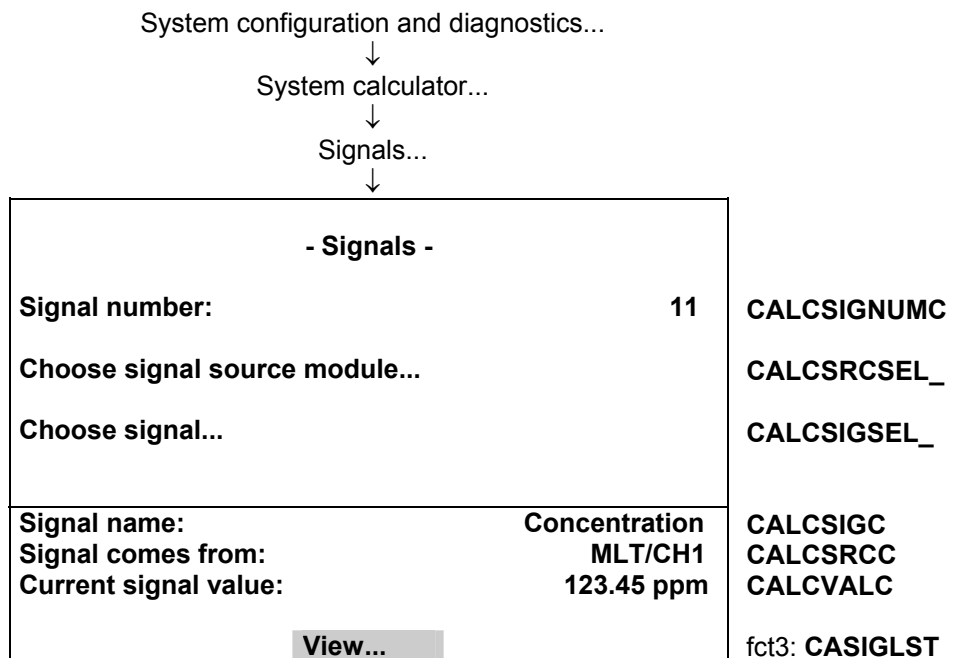
Picture 1-2 : Signal Assignment of System Calculator
