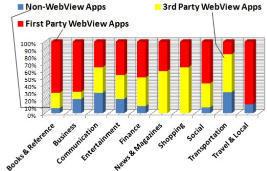
Figure 5: WebView Usage Based On Categories
