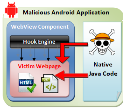
Figure 3: Attack Methods
