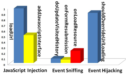
Figure 6: API Usages by Third-Party Apps
