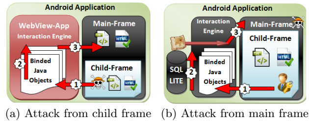
Figure 2: Threat Models
