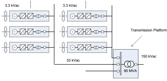
Fig. 4. A 90 MW wind farm with 33 kV ac collection grid
