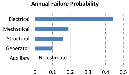
(b) Estimate of probability of types of wind turbine failures in a year [6]
