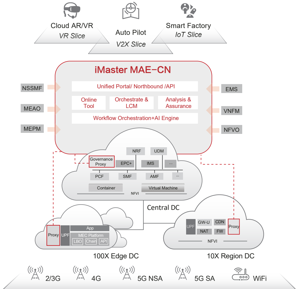
Figure 3-4 Product architecture for applying iMaster MAE to core networks
