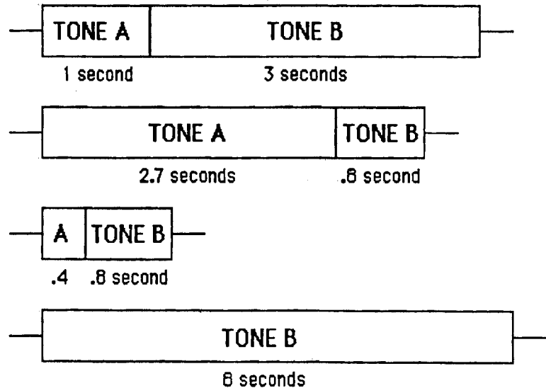
Fig. 6-2. Two-Tone Sequential Timing
