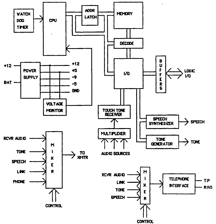
Fig. 9-1. System Diagram
