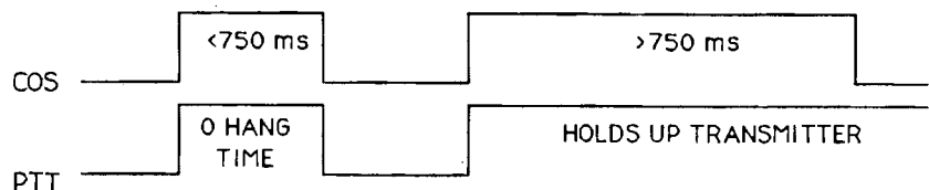
Figure 7-6. Kerchunker Filtering
