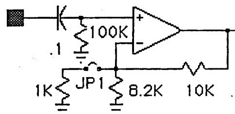
Figure 2-5. Receiver Audio Input (REPEATER Connector, Pin 7, blue)
