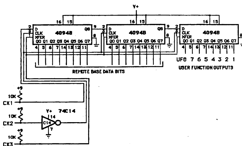
Fig. 8-9. Recovering UF Outputs and Remote Base Frequency Information
