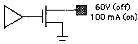
Figure 2-4. PTT Output (REPEATER Connector, Pin 4, orange)
