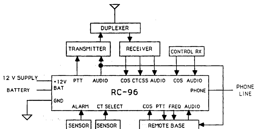
Fig. 7-1. Repeater Block Diagram
