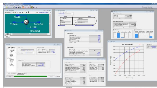
HTRI's XSimOp Shell-Tube is seamlessly integrated within UniSim Design.
