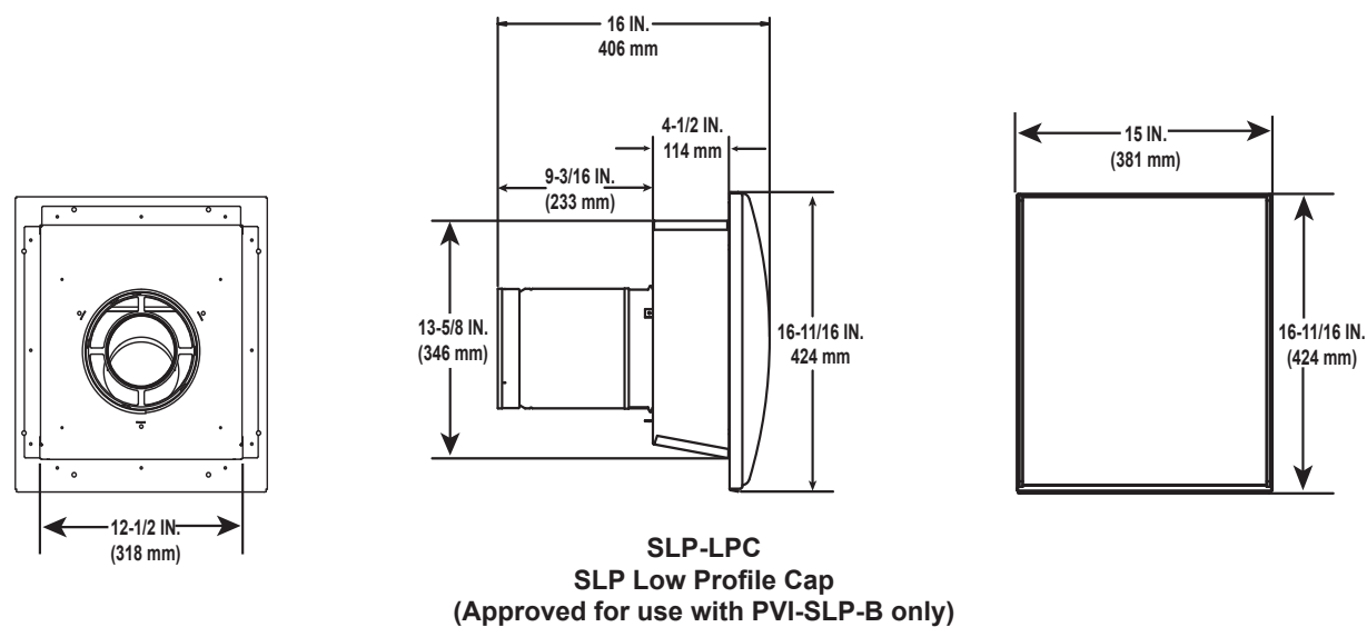
Figure 12.5 PVI-SLP-B Vent Components
