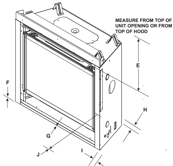
* MINIMUM FRAMING DIMENSIONS
