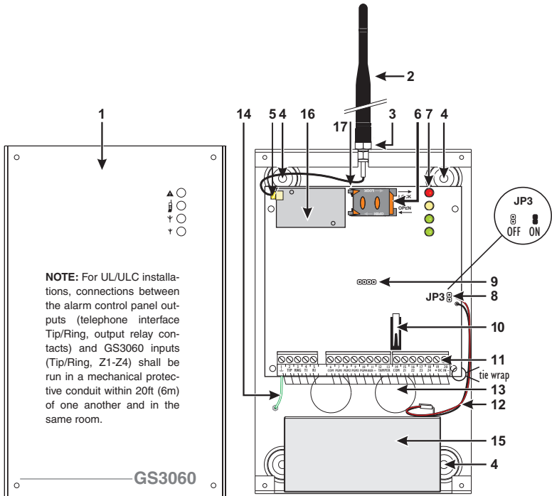
Figure 1 - Parts
