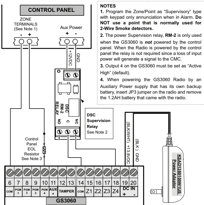
Figure 4 - Power Supply and Supervision Wiring Diagram
