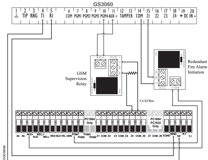
Connection Details for GSM Supervision Relay & Redundant Fire Alarm Transmission
