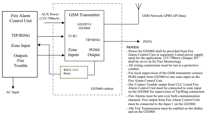
Figure 6 - DSC Subscribers' Unit Fire and GSM Transmitter Mounted in the Same Room
