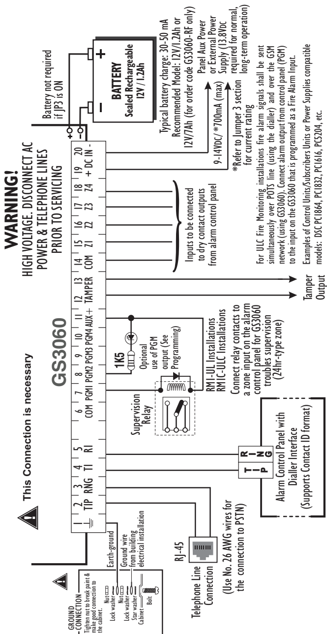
Figure 2 - Wiring Diagram
