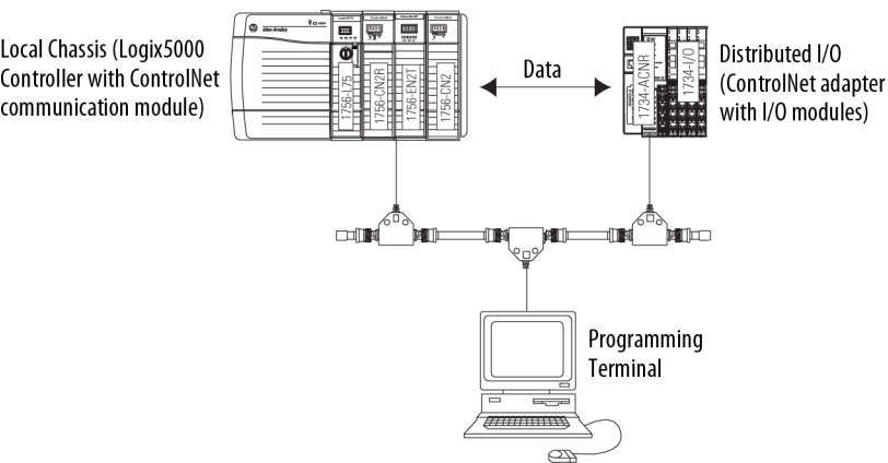
Figure 10 - Overview of ControlNet I/O Distribution
