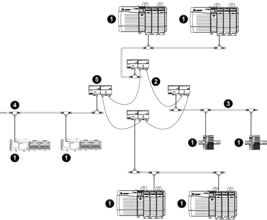
Figure 7 - Example ControlNet Network Ring Topology
