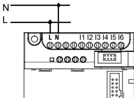
Figure 2.4 AC Type
