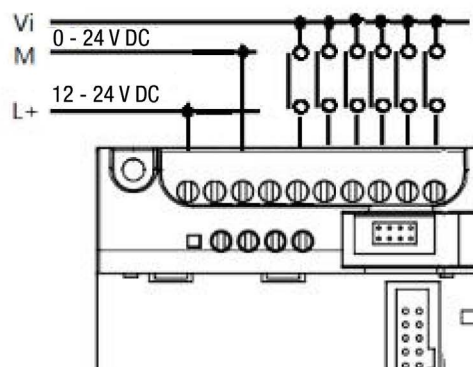
Figure 2.7 DC Type
