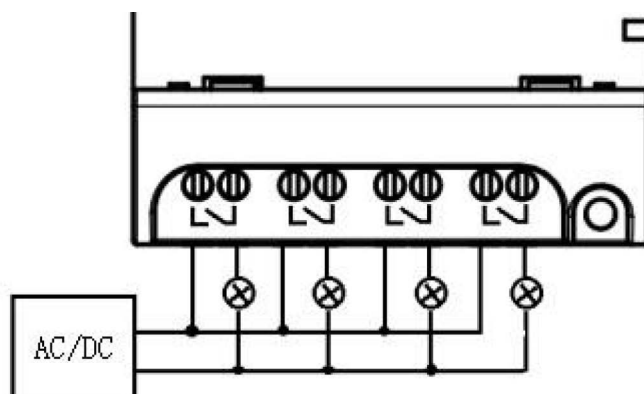
Figure 2.9 Relay output
