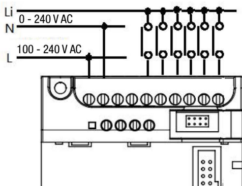
Figure 2.6 AC Type
