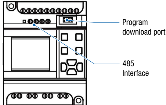
Figure 4.1 Communication connection
