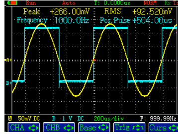
Dual-channel measurement
