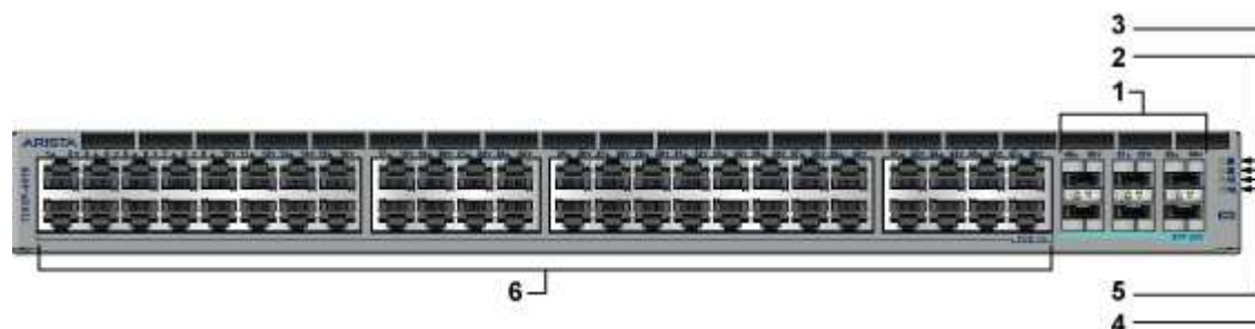
Figure C-3: CCS-720XP-48Y6
