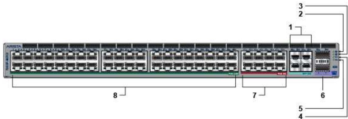
Figure C-1: CCS-720XP-48ZC2
