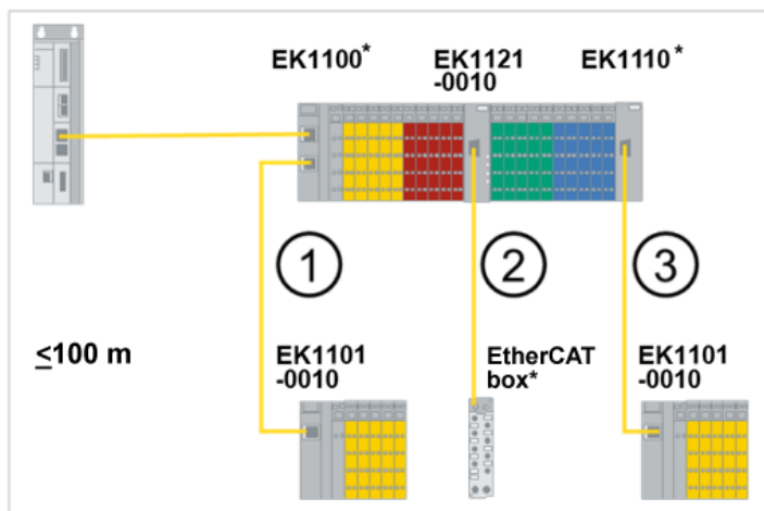
Fig. 11: Topologies with Extended Distance- and Standard components, distances up to 100 m
