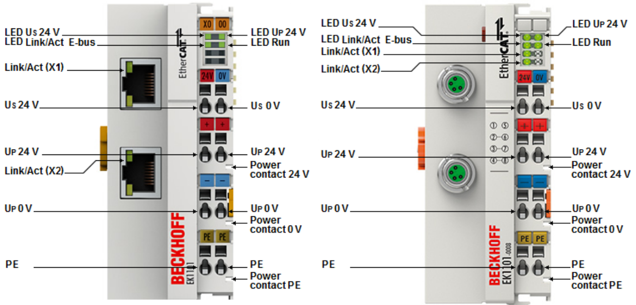
Fig. 65: Diagnostic LEDs EK1101-00x0, EK1101-0008
