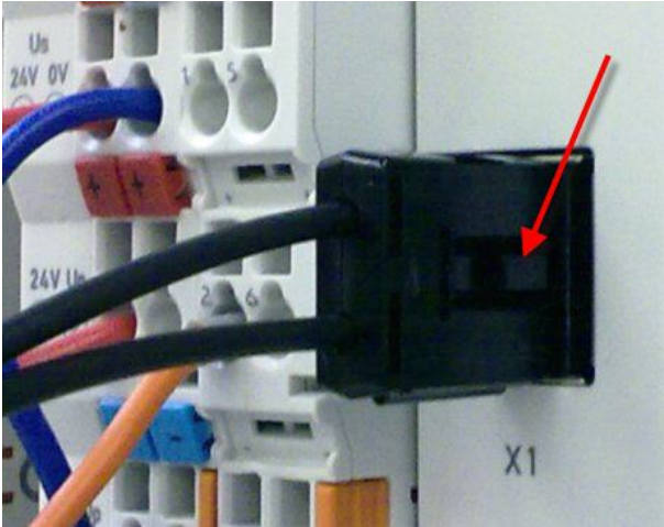
Fig. 55: Latching lug with release catch on the POF duplex plug
