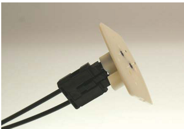
Fig. 61: Sanding gauge with protruding fiber ends
