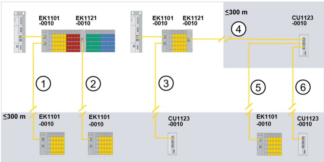
Fig. 9: Topologies with Extended Distance components, distances up to 300 m
