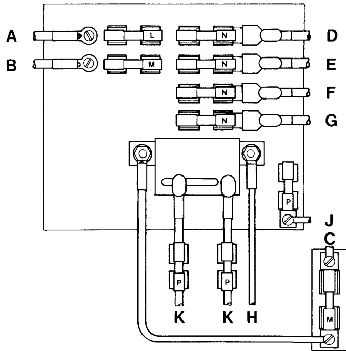
Low Voltage Distribution Panel
