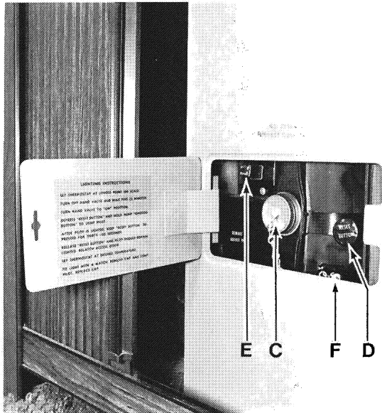
Furnace Controls (23-31 Ft.)
