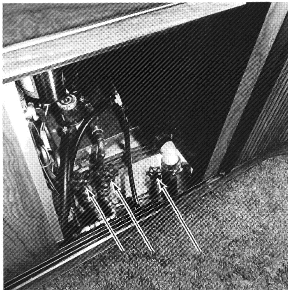
Water Drain Valves Galley (Int'l.)
