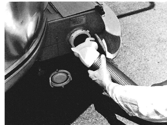
Waste Drain Hose Hook-Up
