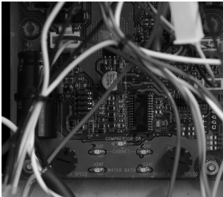
FIG 14 Temperature LEDs JDF-2S (Early Models)
