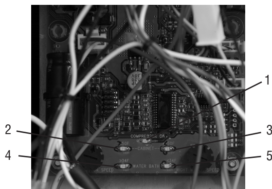
FIG 17 JDF-2S (Early Models)
