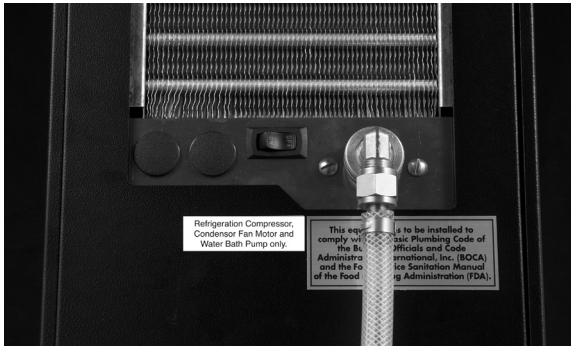
FIG 7 Refrigeration Switch - JDF-2S Early Models
