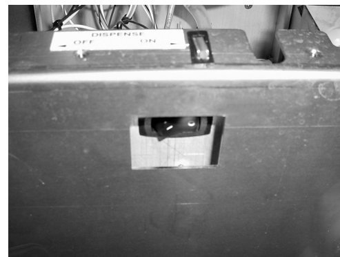
FIG 13 Dispense Lockout Switch
