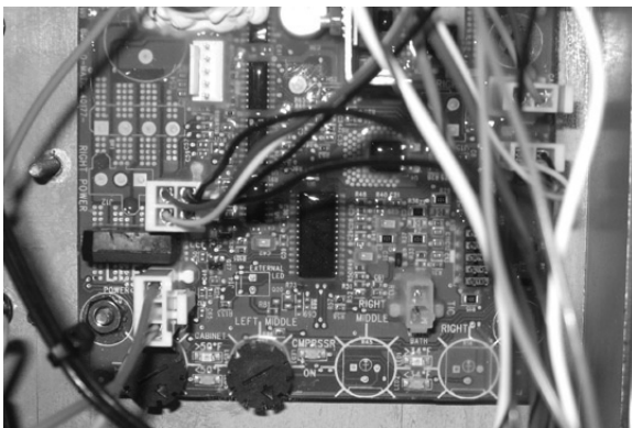
FIG 14A Temperature LEDs JDF-2S (Late Models)
