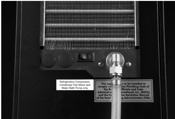
FIG 1 Plumbing Connections - JDF-2S
