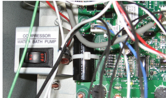
FIG 7A Refrigeration Switch - JDF-2S Late Models
