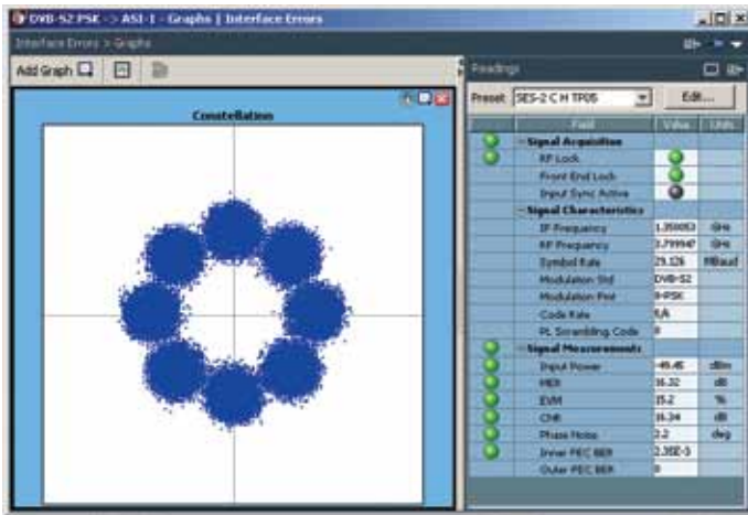
Figure 3.3. DVB-S2 8PSK signal with high amounts of noise, but enough Forward Error Correction to provide a quasi-error-free transport stream.
