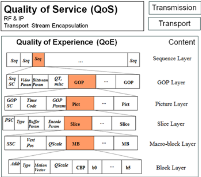
Figure 2.2. QoS and QoE layers.
