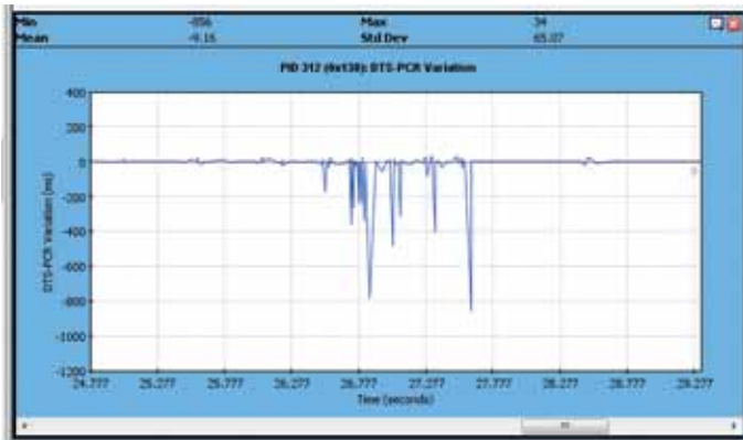
Figure 3.20. Cable headend encoder generating negative DTS-PCR delta values (should be impossible).
