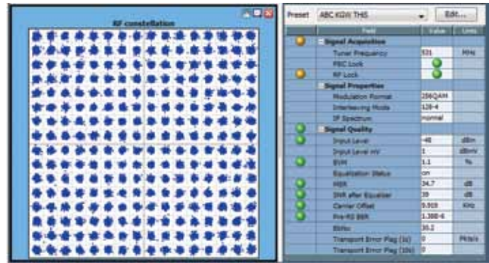
Figure 3.4. 256 QAM cable TV signal.
