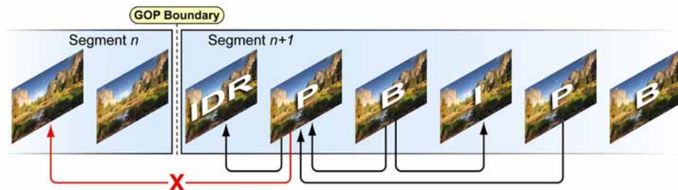
Figure 1.8. H.264 compressed video content with Groups of Pictures (GOP) made up of I, P, and B frames. An Instantaneous Decoder Refresh (IDR) frame follows each GOP boundary. Frames in segment n+1 cannot reference previous segments.
