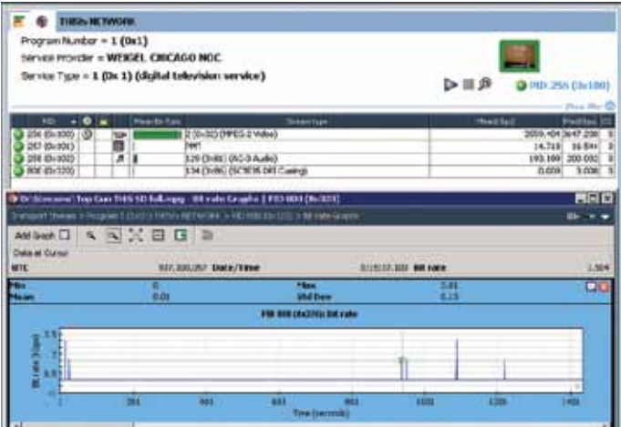
Figure 3.23. PID 800 DPI packets arrive about every 15 minutes.
