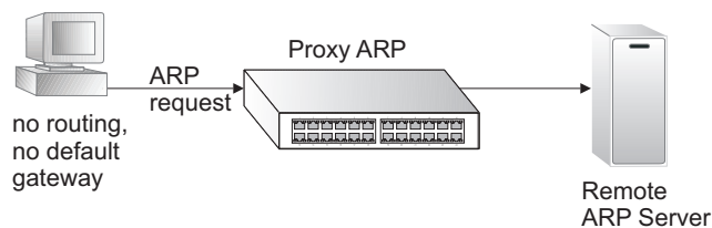
Figure 381: Proxy ARP
