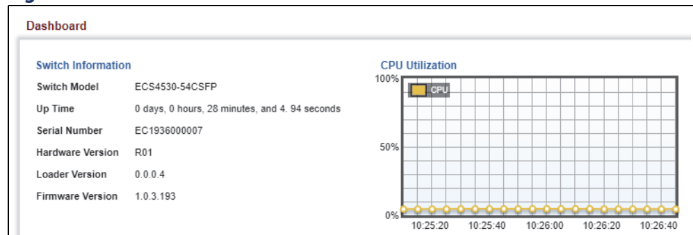
Figure 1: Dashboard
