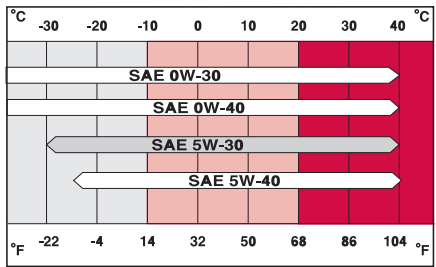
Viscosity chart
