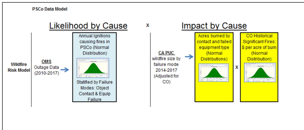
Figure SDR-D-6: Wildfire Risk Model Process
