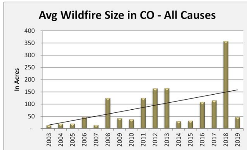
Figure SDR-D-5: Average Colorado Wildfire Size (2003-2019)
