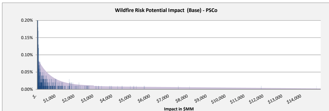
13 Figure SDR-D-7: Wildfire Risk Model Monte Carlo Simulation
