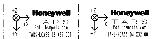
FIGURE 4. MARKING INFORMATION
