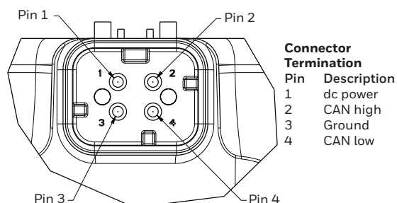
FIGURE 3. PINOUT
