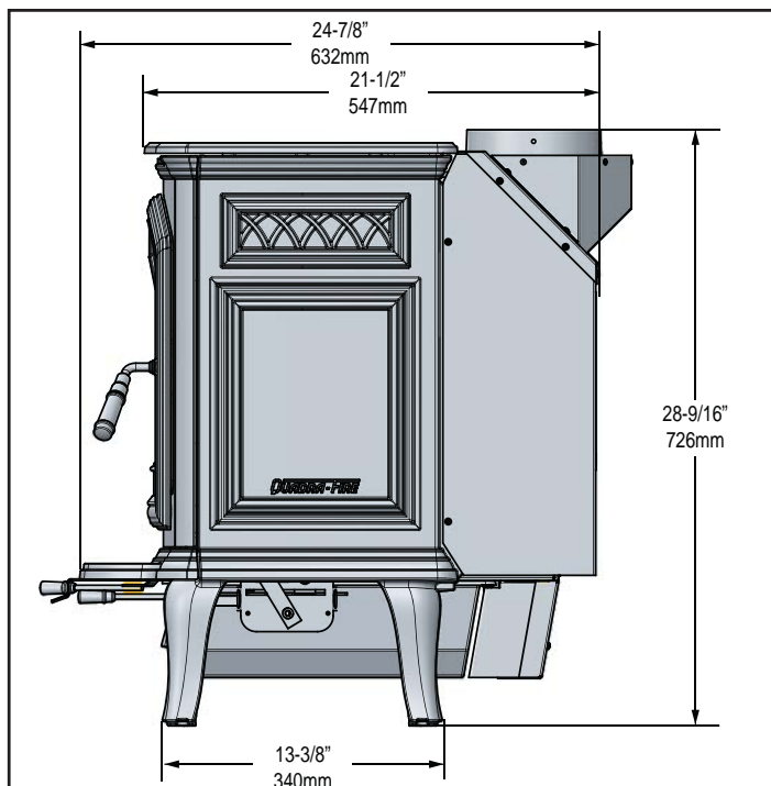
Figure 7.2 Side View with vertical flue
