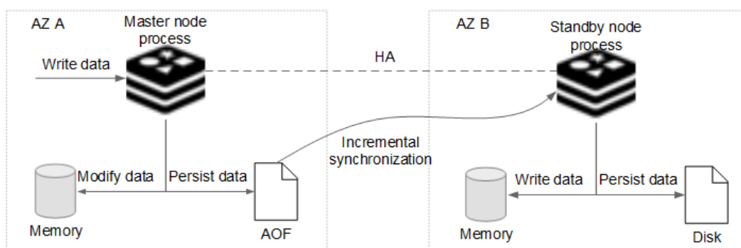
Figure 1-12 Cross-AZ deployment of a master/standby DCS instance
