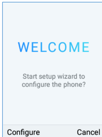
Figure 6: Setup wizard
