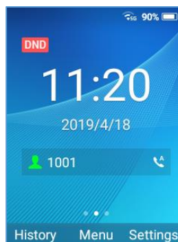
Figure 54: DND Enabled
