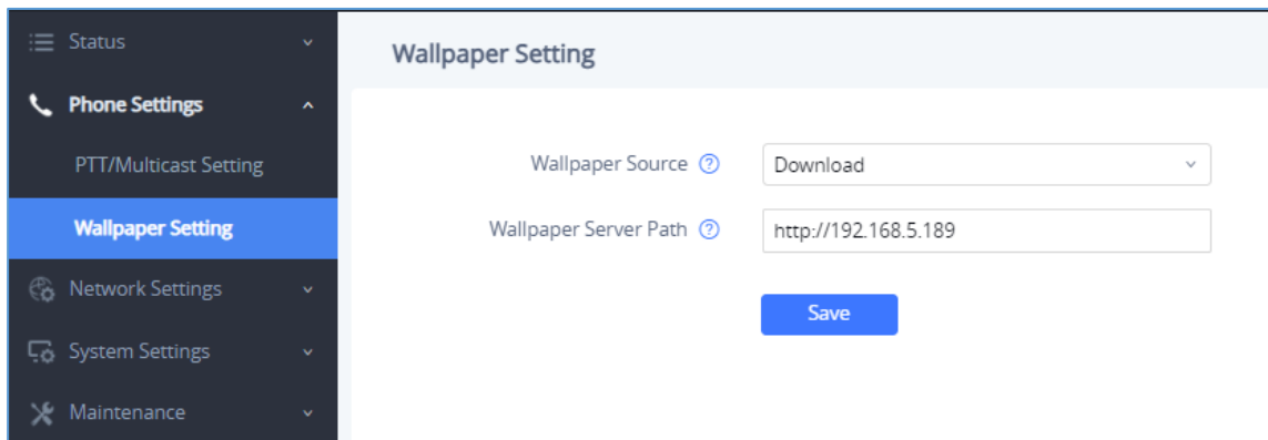
Figure 43: Wallpaper – Download
