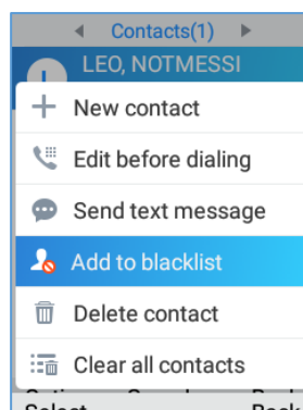
Figure 75: Blacklist
