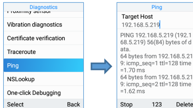
Figure 107: Ping
