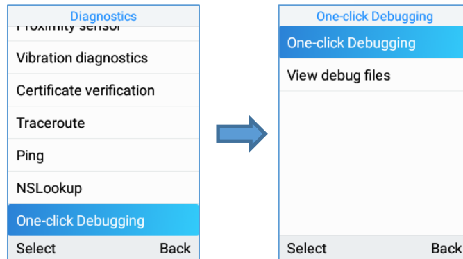
Figure 109: one-click debugging
