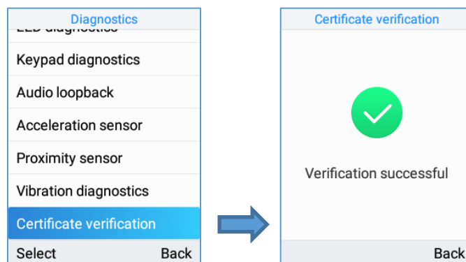
Figure 105: Certificate Verification
