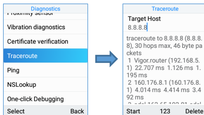
Figure 106: Traceroute
