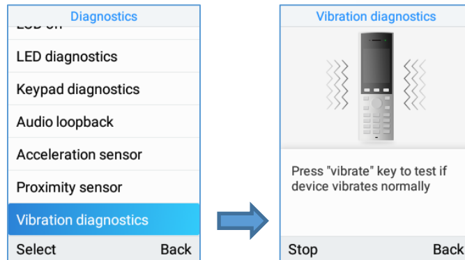
Figure 104: Vibration diagnostics
