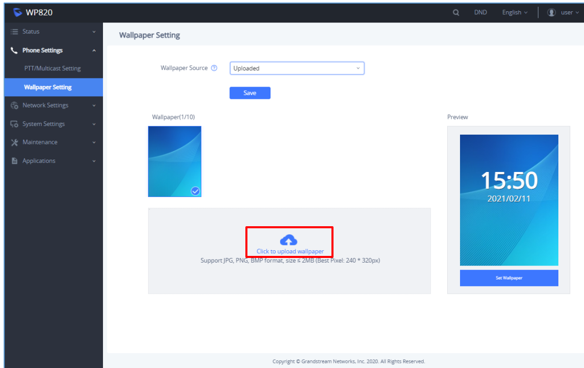
Figure 40: Wallpaper Settings
