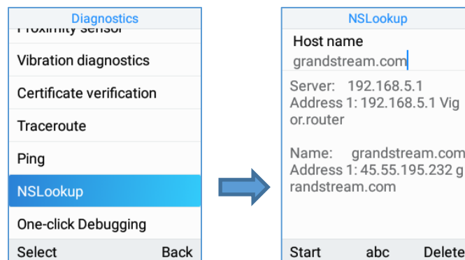
Figure 108: Nslookup
