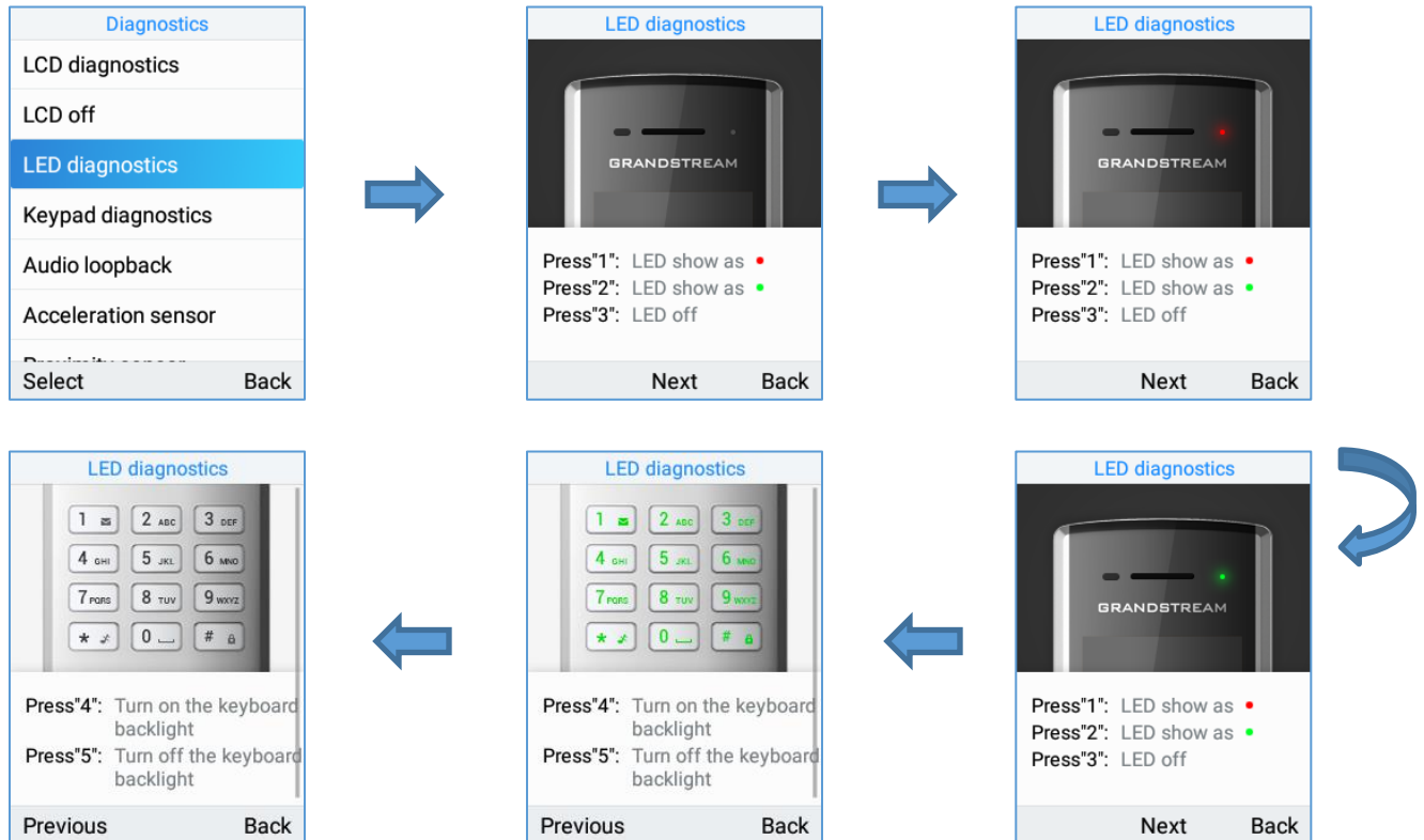
Figure 99: LED Diagnostics
