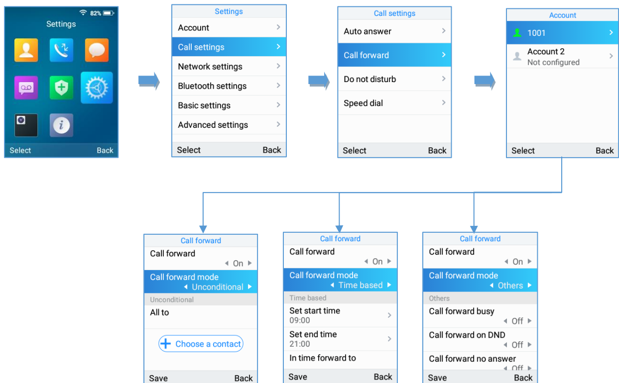
Figure 55: Call Forwarding
