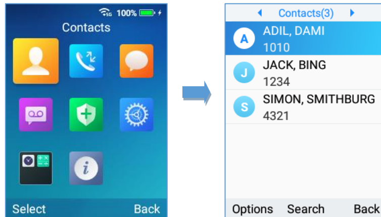
Figure 72: Accessing Contacts
