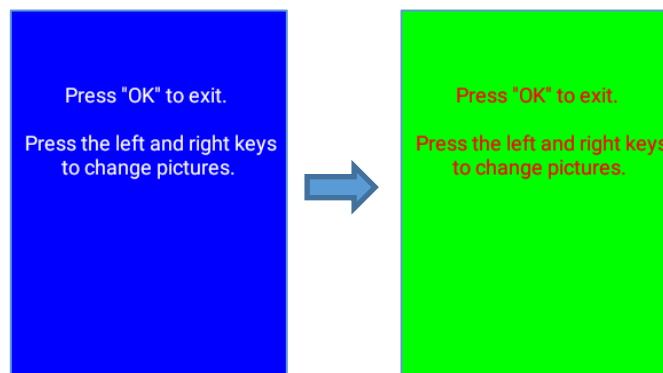
Figure 97: LCD Diagnostics
