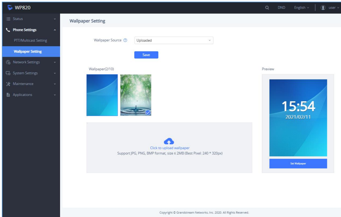
Figure 42: Wallpaper – Uploaded
