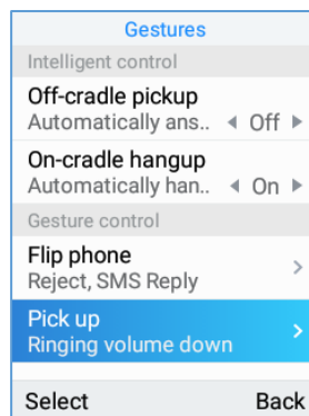
Figure 93: Pick up
