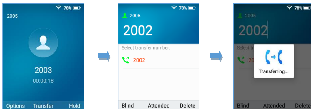
Figure 56: Blind Transfer
