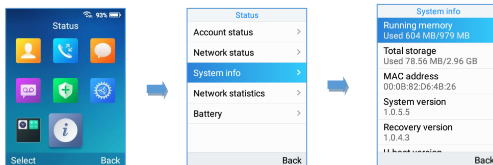
Figure 23: System Info
