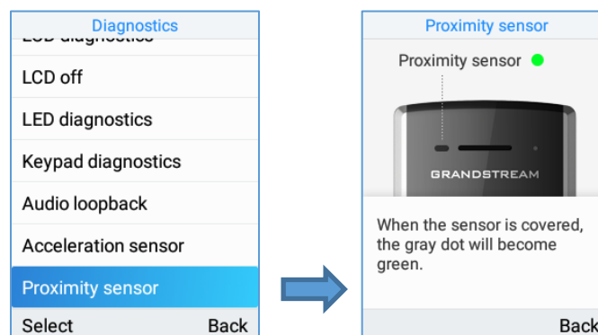
Figure 103: Proximity sensor
