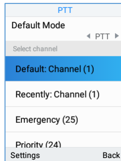
Figure 84: PPT Channel
