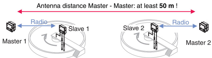
Fig. 3-8 Example 1: Maximum distance of the MIQ/Blue PS masters
