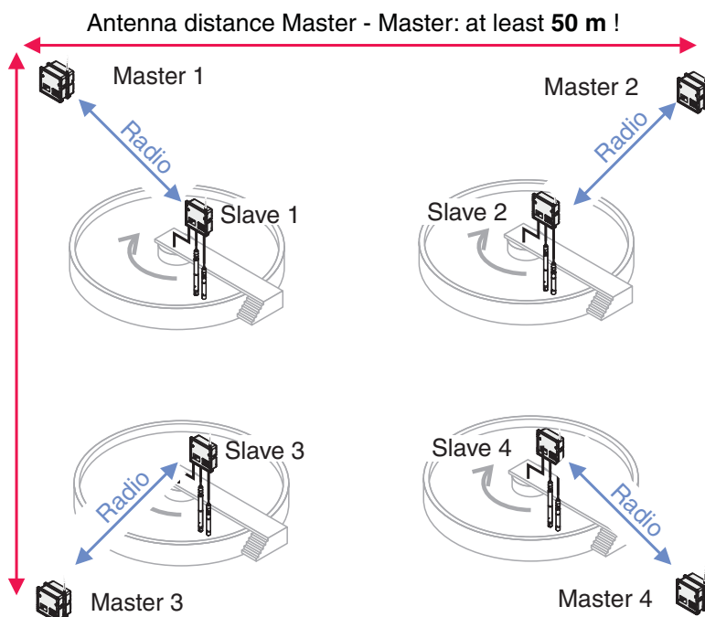
Fig. 3-9 Example 2: Maximum distance of the MIQ/Blue PS masters
