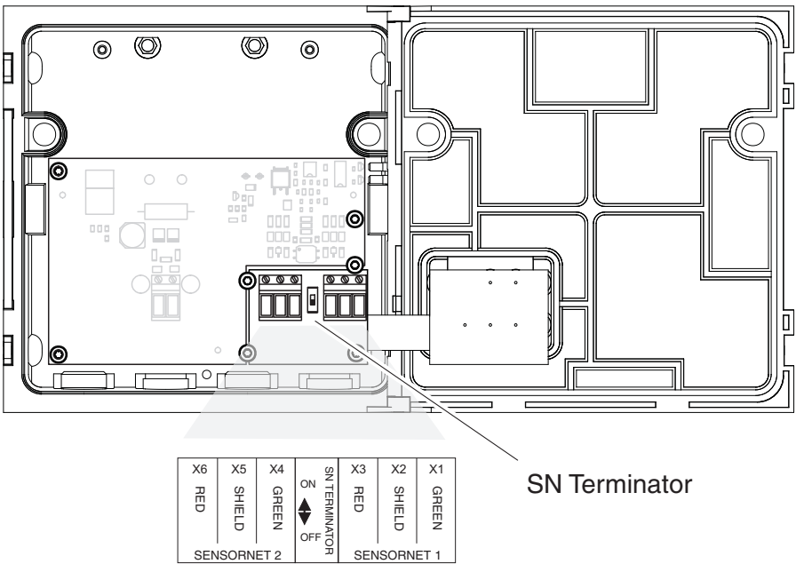
Fig. 3-1 Correct setting of the terminator switches
