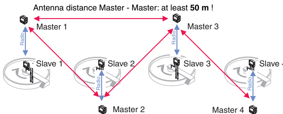
Fig. 3-10 Example 3: Maximum distance of the MIQ/Blue PS masters
