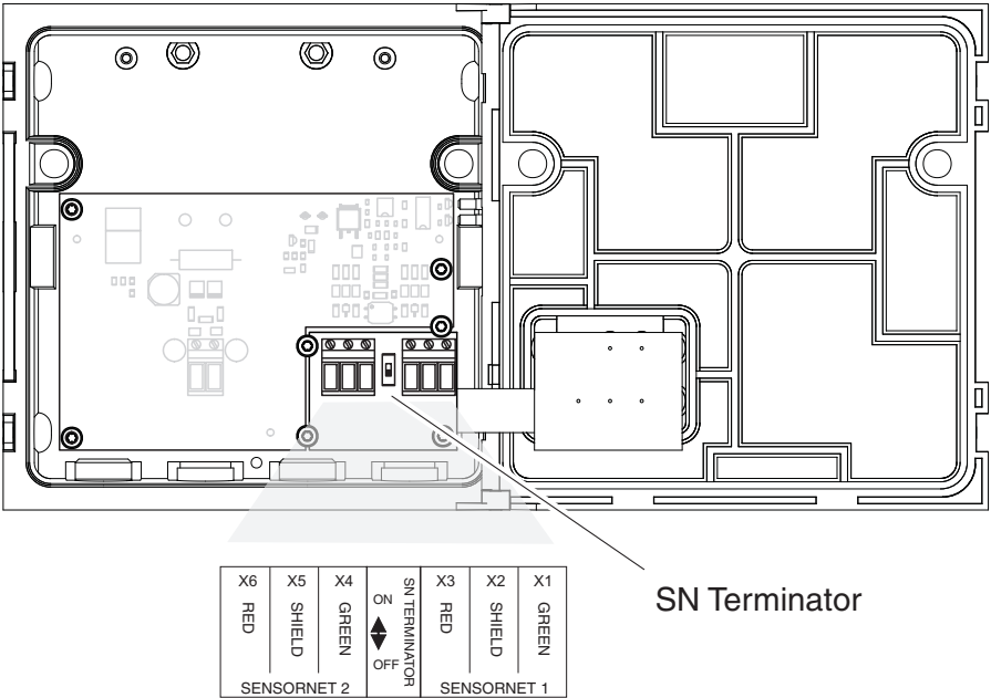
Fig. 3-3 Terminator switch
