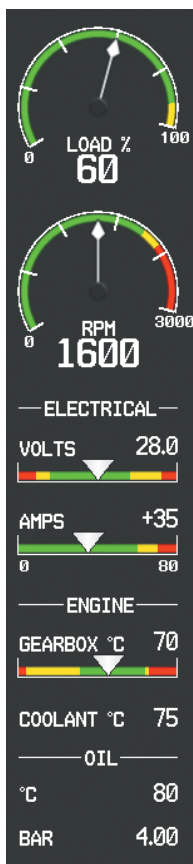
Engine System Display on the MFD
