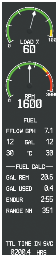
Engine Fuel Display on the MFD
