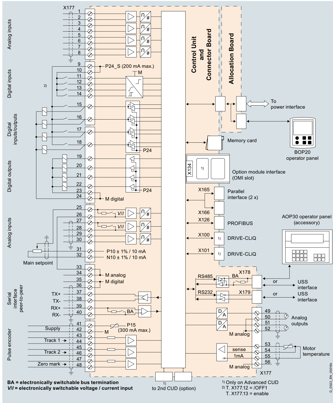
Connection diagram, Standard CUD/Advanced CUD with typical connections
