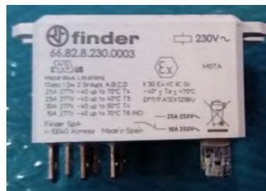
Sealed Relay ATEX Rated
