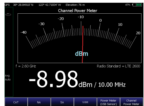
Easily measure power levels using the built-in channel power meter
