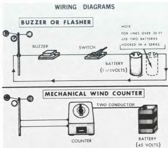
Figure 31.12—Wiring diagrams: upper, for buzzer or flasher; lower, for mechanical wind counter.
