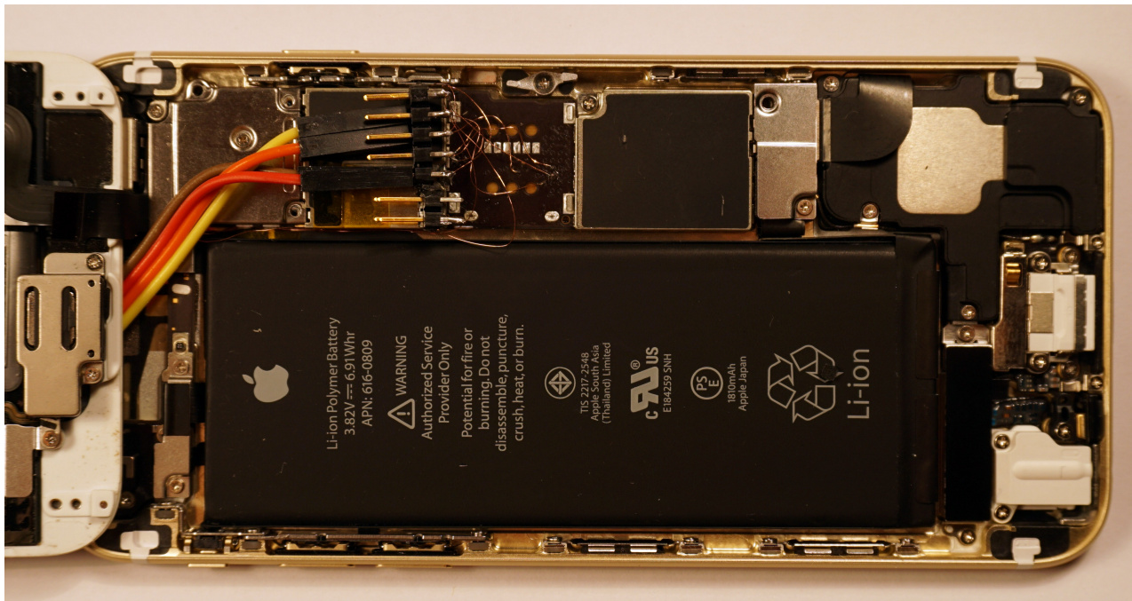
Above: image of the UART and GPS sync probing experiment. The majority of the test points are located underneath the SIM card connector, which was removed for this experiment.
