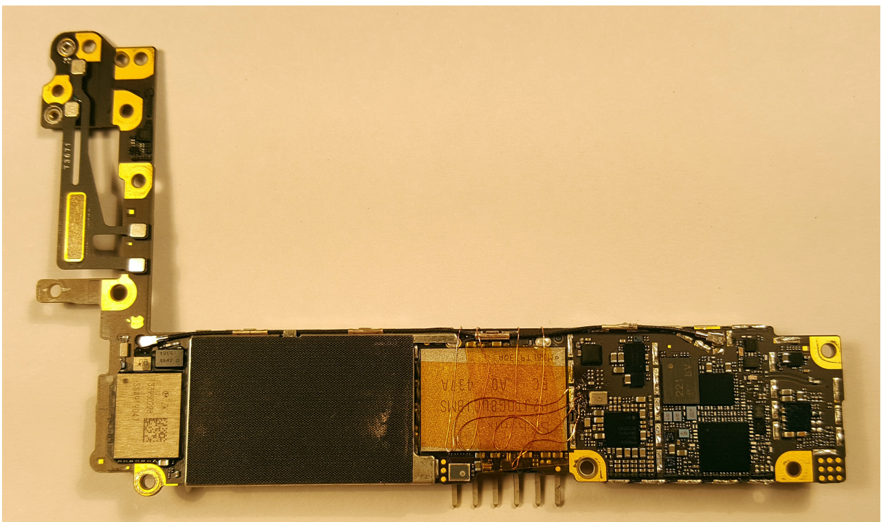
Above: image of the backside of the FE1, FE2 probe experiment. The test points are located adjacent to the NAND Flash, underneath an RF shield which was removed for this experiment. The test points were covered with soldermask, which was removed through mechanical abrasion.
