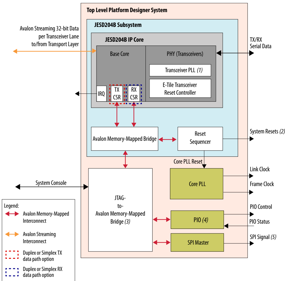
Figure 11. Platform Designer System for System Console Control Design Example for Intel Stratix 10 E-Tile Devices
