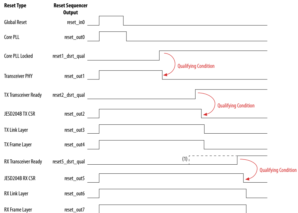
Figure 14. Reset Sequence
