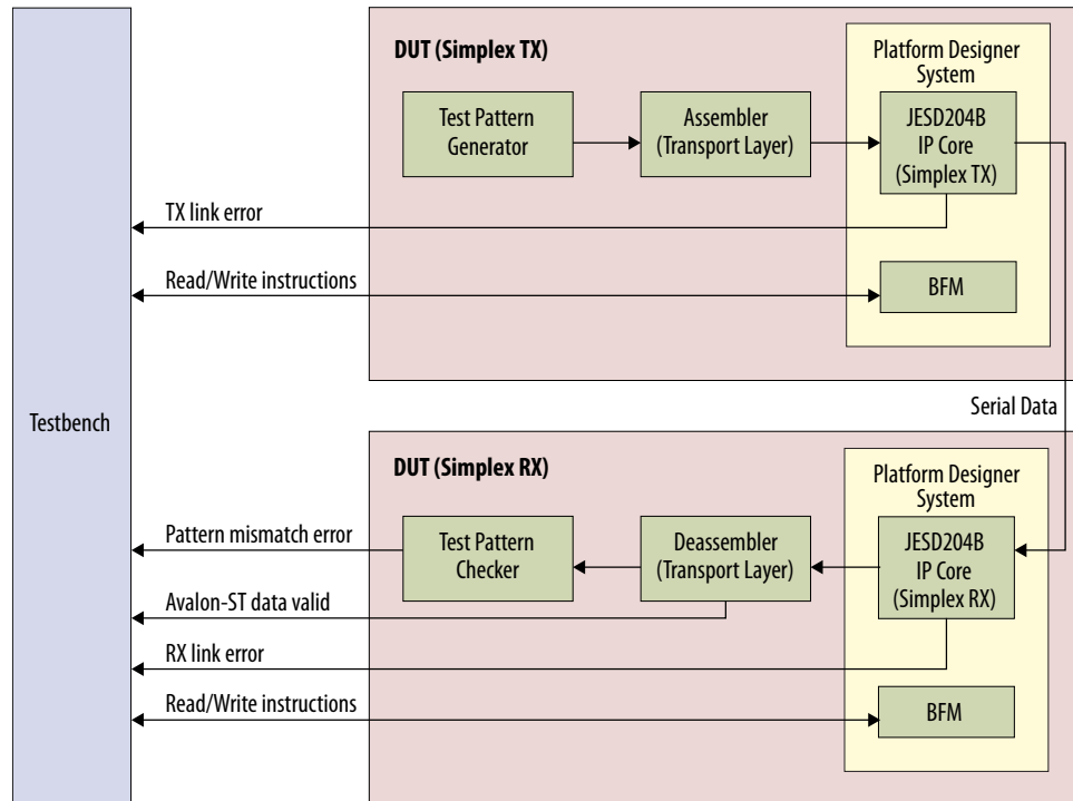
Figure 17. Simulation Testbench Block Diagram (Simplex TX or RX)
