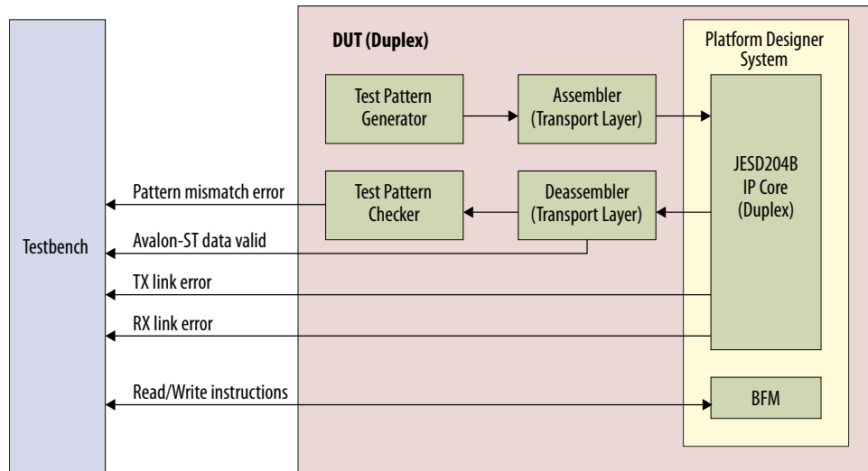
Figure 18. Simulation Testbench Block Diagram (Duplex)
