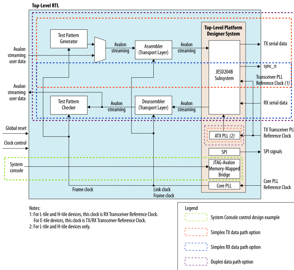
Figure 9. JESD204B Design Example Block Diagram
