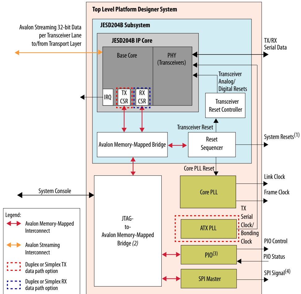
Figure 10. Platform Designer System for System Console Control Design Example for Intel Stratix 10 L-Tile and H-Tile Devices
