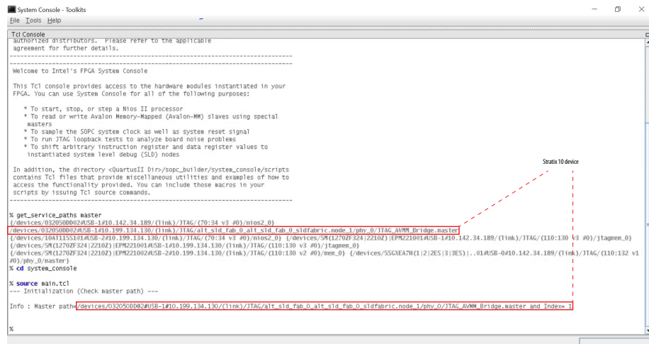
Figure 7. Source main.tcl
