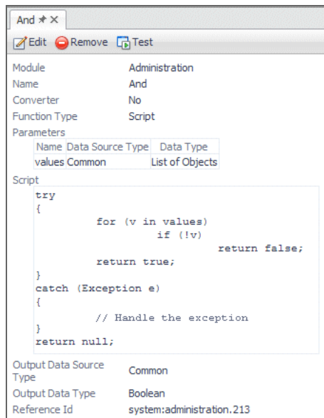
Figure 34. Script function example
