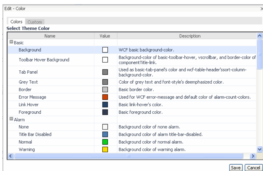
Figure 37. Themes
