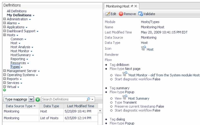
Figure 21. Type mappings
