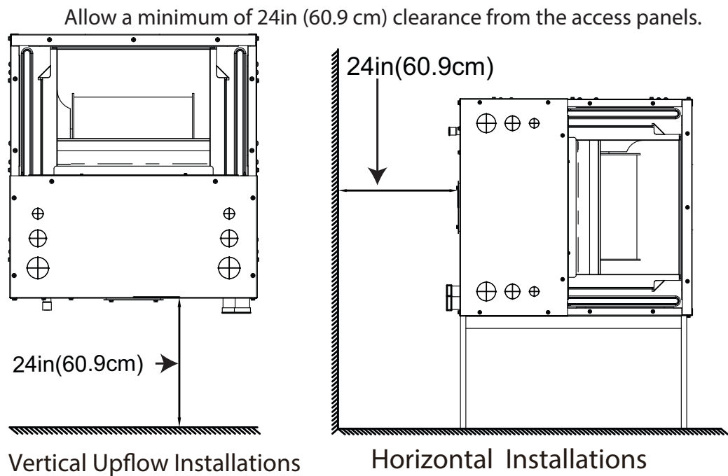
Fig. 4 — Clearances
