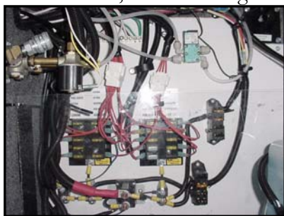
Figure 7-2. 12 VDC Fuse Panels
