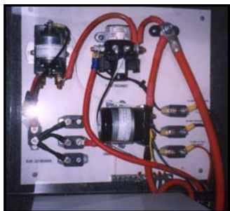
Figure 7-18. Resettable Circuit Breakers
