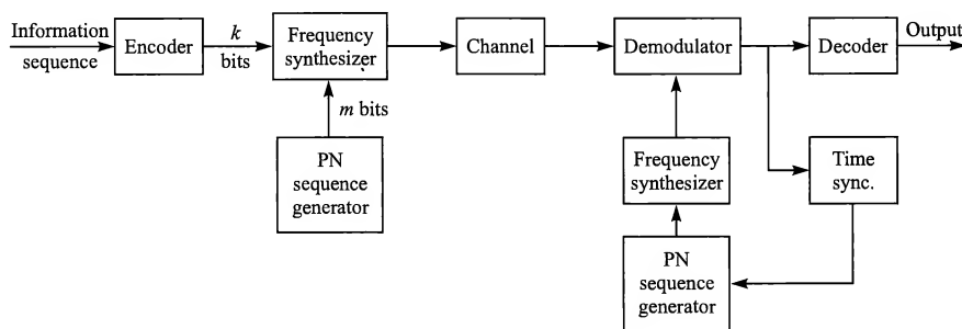
FIGURE 12.3-3 Block diagram of an independent tone FH spread spectrum system.
