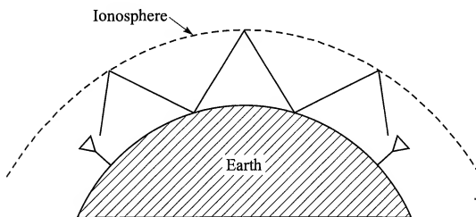
FIGURE 1.2–4 Illustration of sky-wave propagation.
