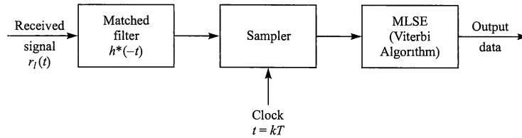
FIGURE 9.3–1 Optimum receiver for an AWGN channel with ISI.
