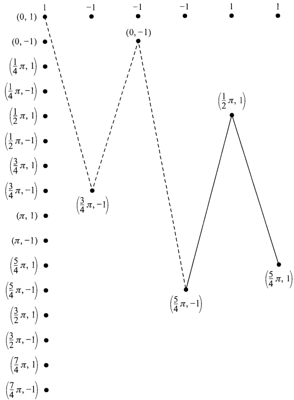
FIGURE 4.9–2 A single signal path through the trellis.
