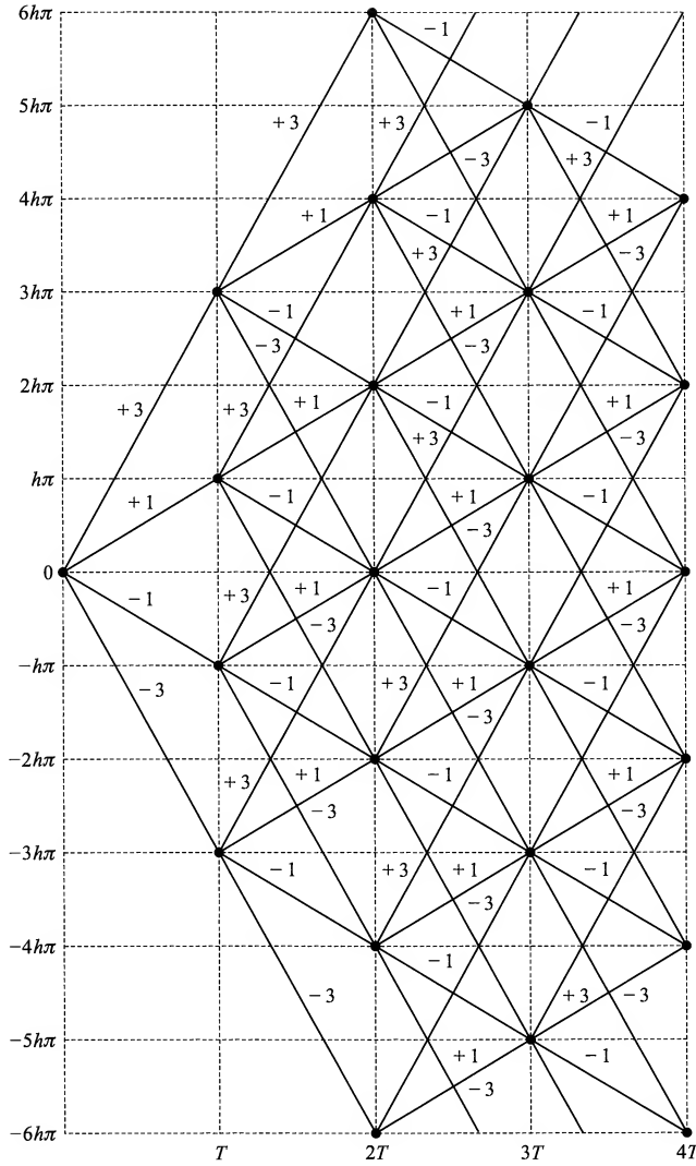
FIGURE 3.3-6 Phase trajectory for quaternary CPM.
