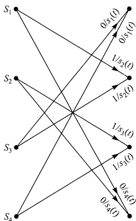
FIGURE 4.8-2 One stage of trellis diagram for delay modulation.
