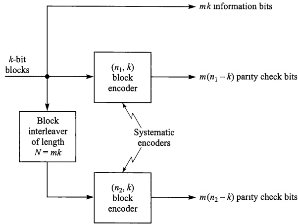
FIGURE 7.13–4 Parallel concatenated block code (PCBC) with interleaver.
