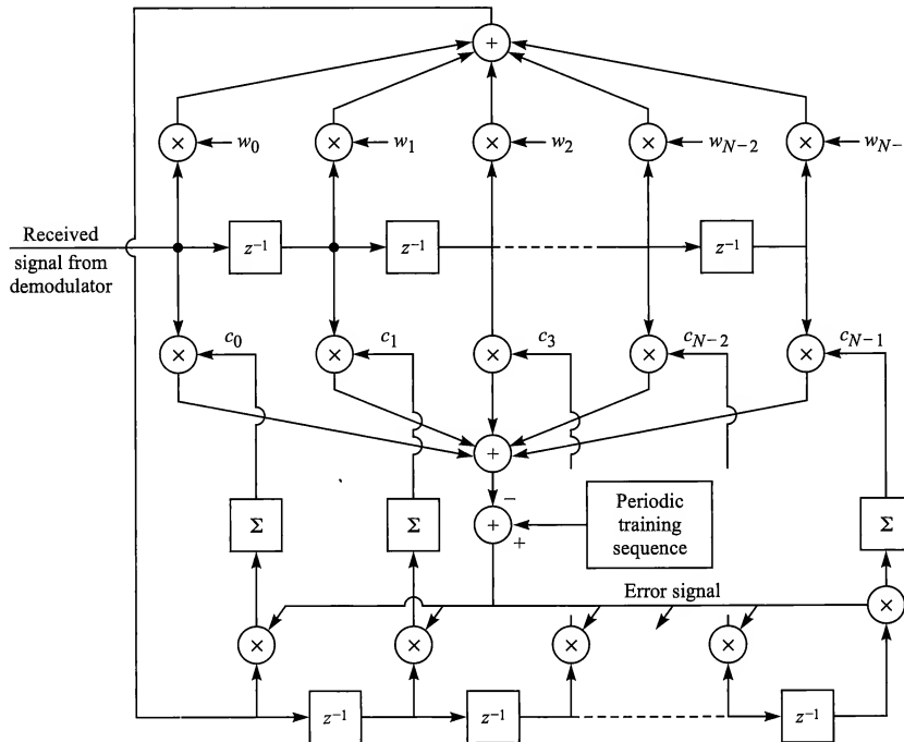
FIGURE 10.1–6 Fast start-up technique for an adaptive equalizer.
