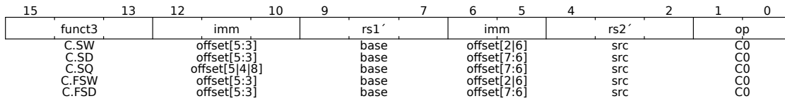
Figure 70: Register-Based Stores
