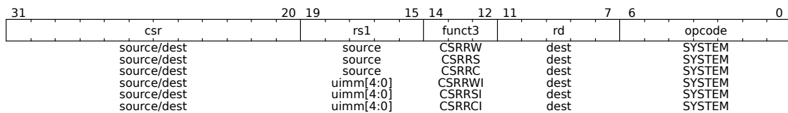
Figure 83: Zicsr Instructions
