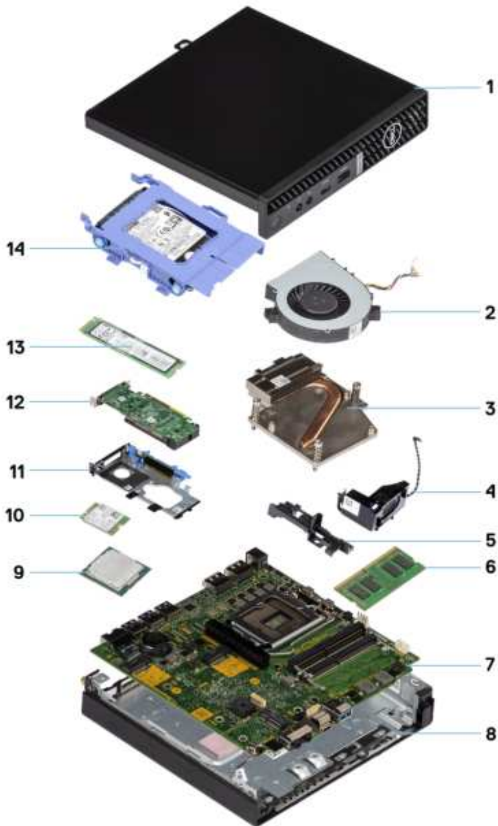
1. Side cover
