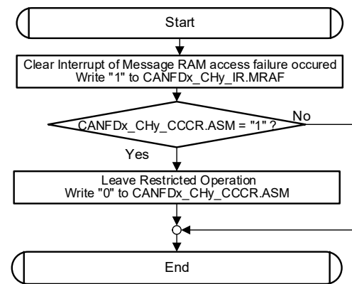
Figure 24-45. Message RAM Access Failure Handling
