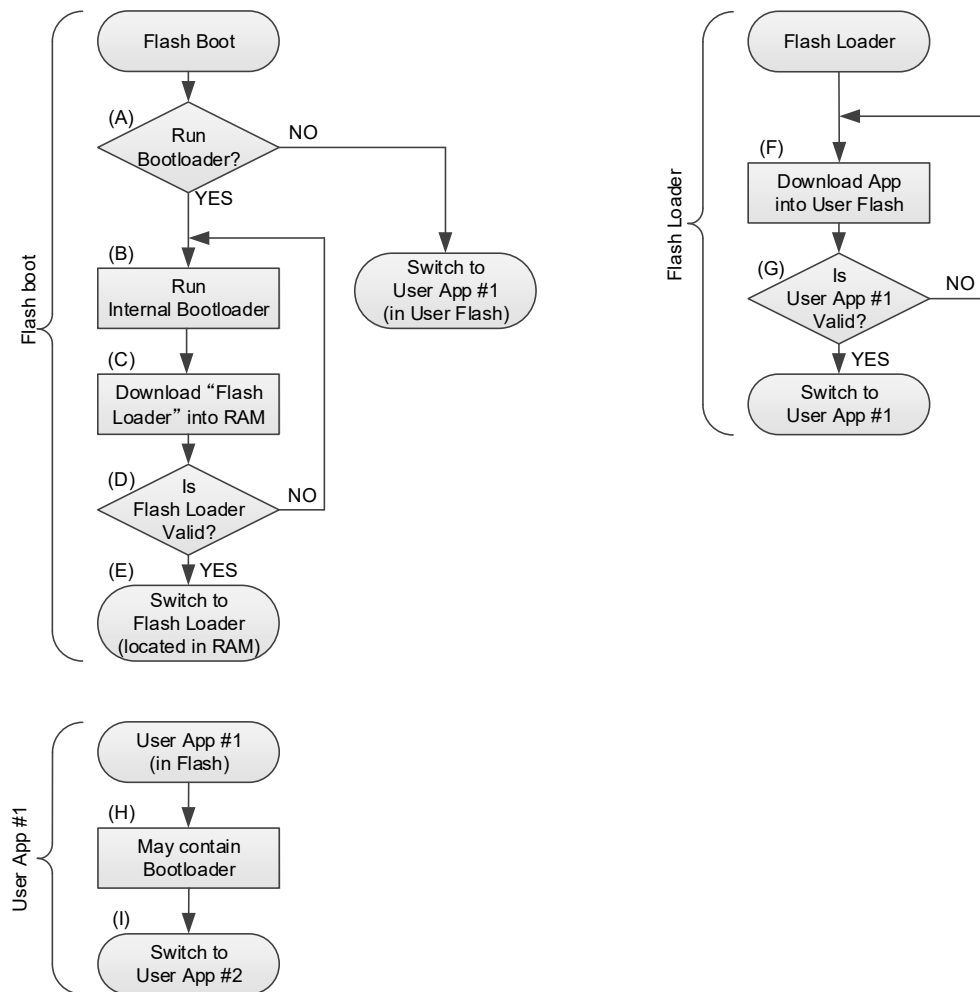
Figure 38-16. Startup and Bootloading Sequence
