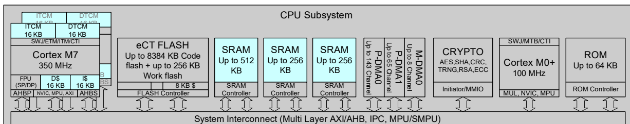
CPU System Block Diagram
