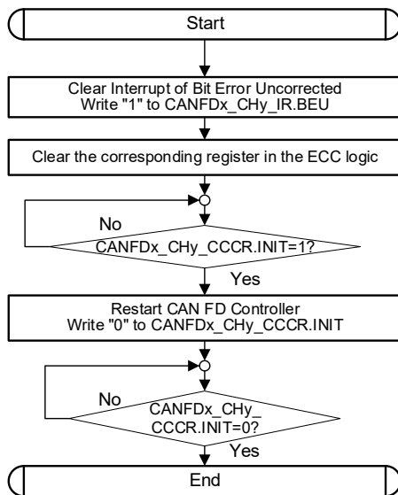
Figure 24-44. Bit Error Handling
