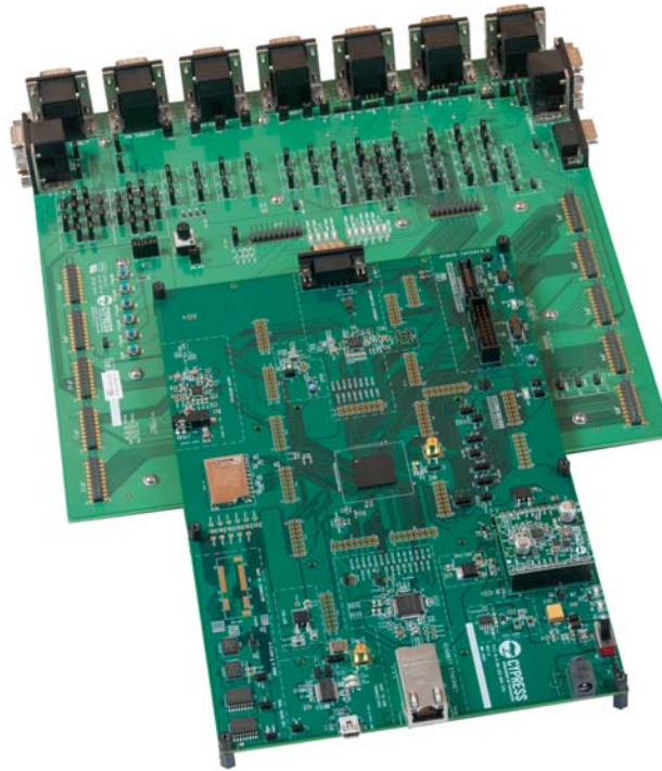
Figure 2-1. Evaluation Board Hook Up with 320-BGA CPU Board
