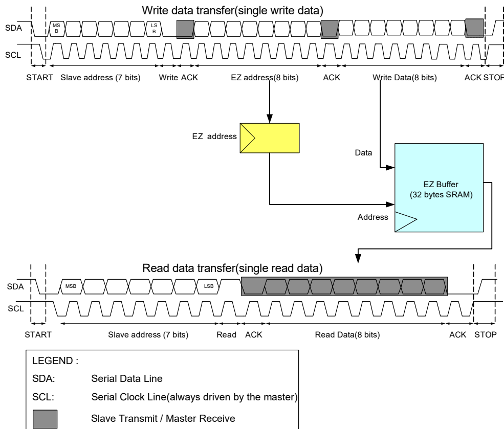
Figure 23-46. EZI 2 C Write and Read Data Transfer
