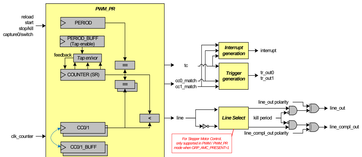
Figure 25-63. PWM_PR Functionality
