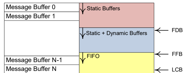
Figure 30-19. Assignment of Message Buffers
