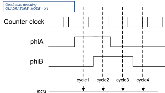
Figure 25-23. phiA/phiB Detection at Counter Clock
