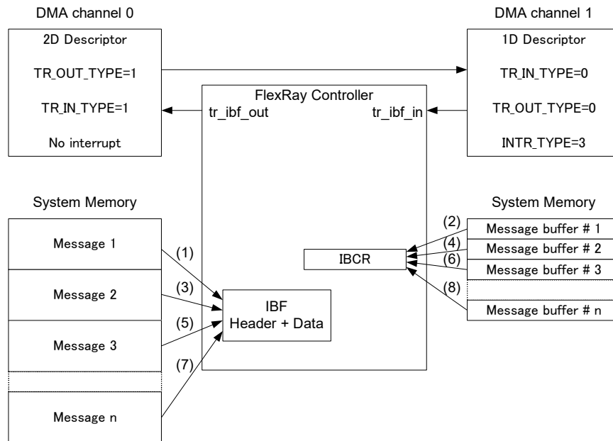
Figure 30-21. DMA Channel Configuration for Input Buffer Access (IBCR only)
