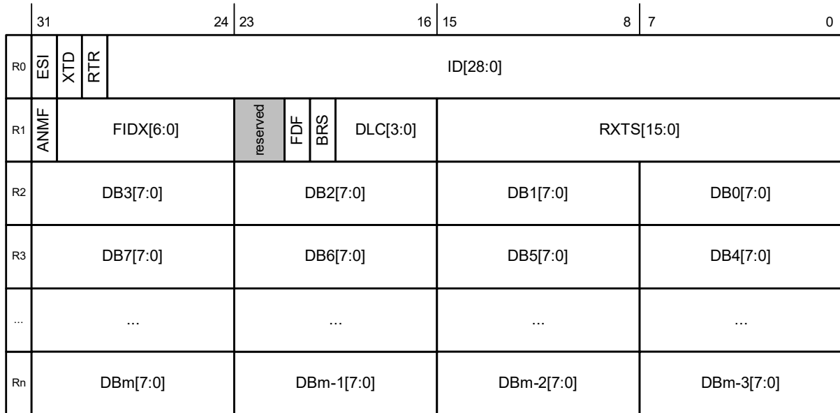
Figure 24-18. RX Buffer and FIFO
