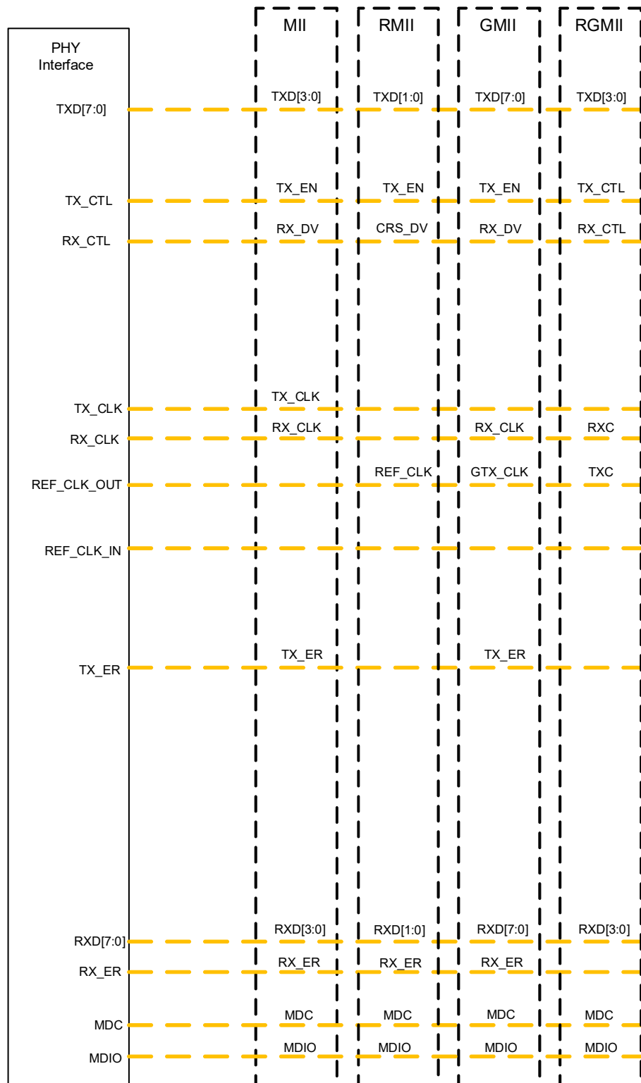
Figure 31-3. PHY Interface
