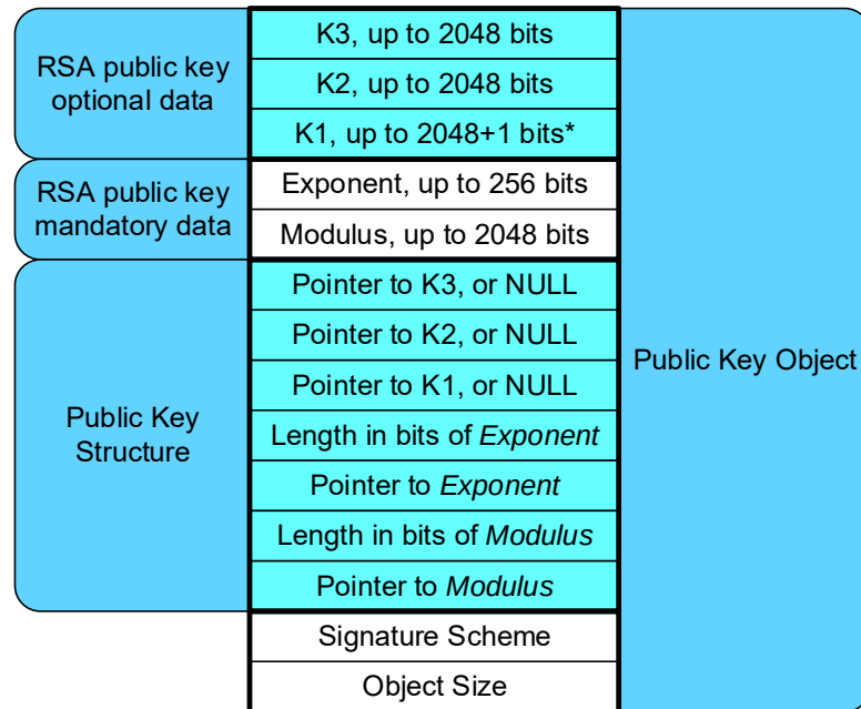
Figure 38-14. Public Key Format
