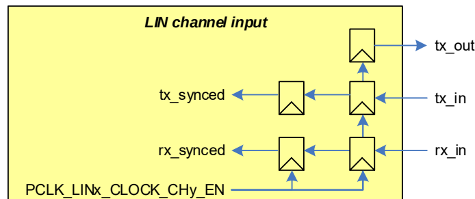
Figure 26-9. LIN Signal Line Synchronization Block Diagram
