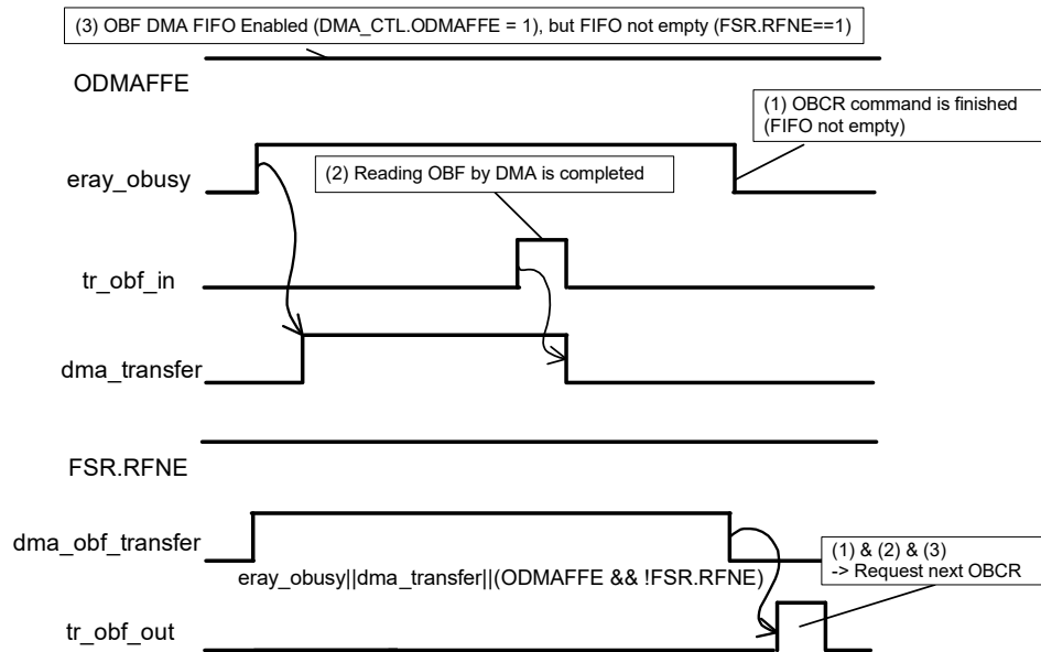
Figure 30-28. Case 3: Receive FIFO is Not Empty after OBCR
