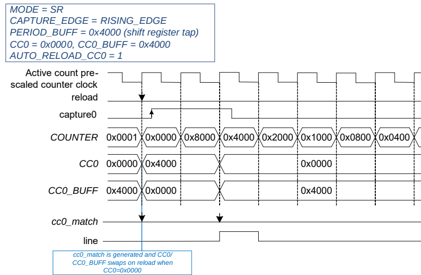
Figure 25-67. SR Shift when PERIOD_BUFF = 0x4000
