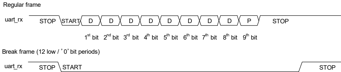
Figure 23-25. UART - Regular Frame and Data Frame
