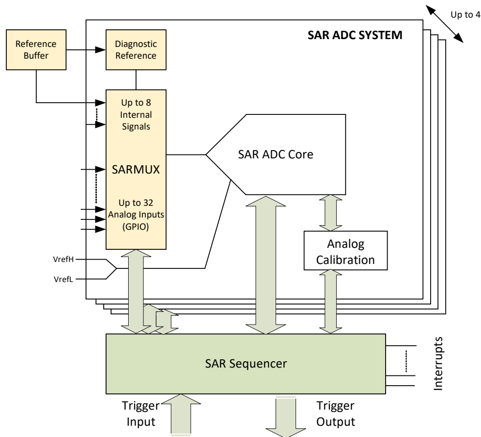
Figure 35-1. SAR ADC System Block Diagram
