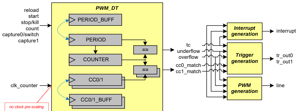
Figure 25-60. PWM with Dead Time Functionality
