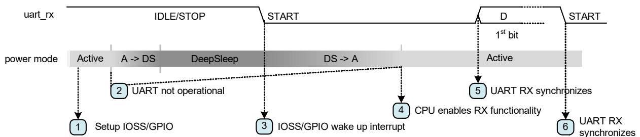
Figure 23-24. UART Start Skip and Wakeup from DeepSleep
