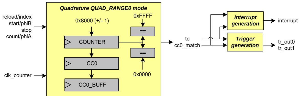
Figure 25-24. Quadrature (QUAD_RANGE0 mode) Function Diagram
