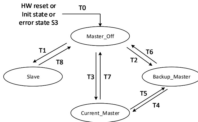
Figure 24-27. Level 0 Master to Slave Relation
