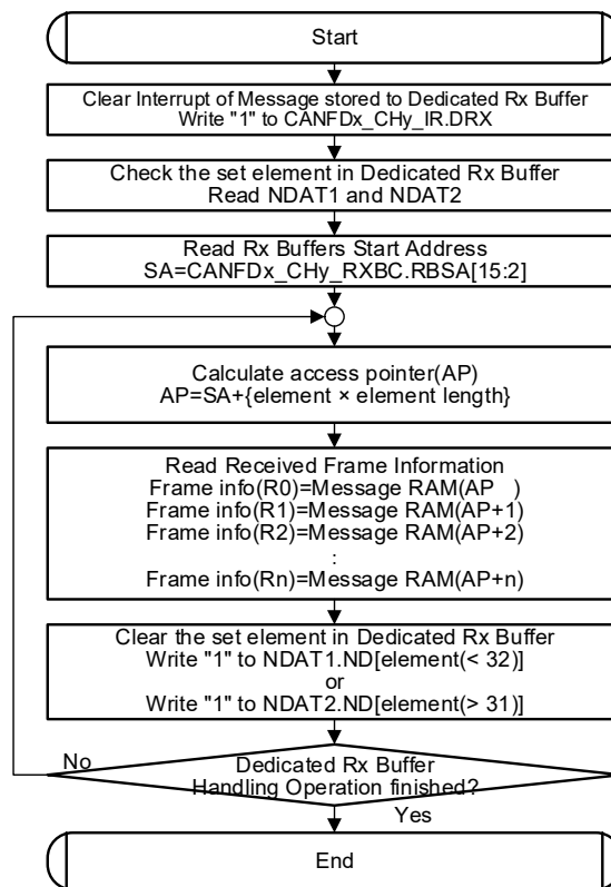
Figure 24-47. Dedicated RX Buffer Handling
