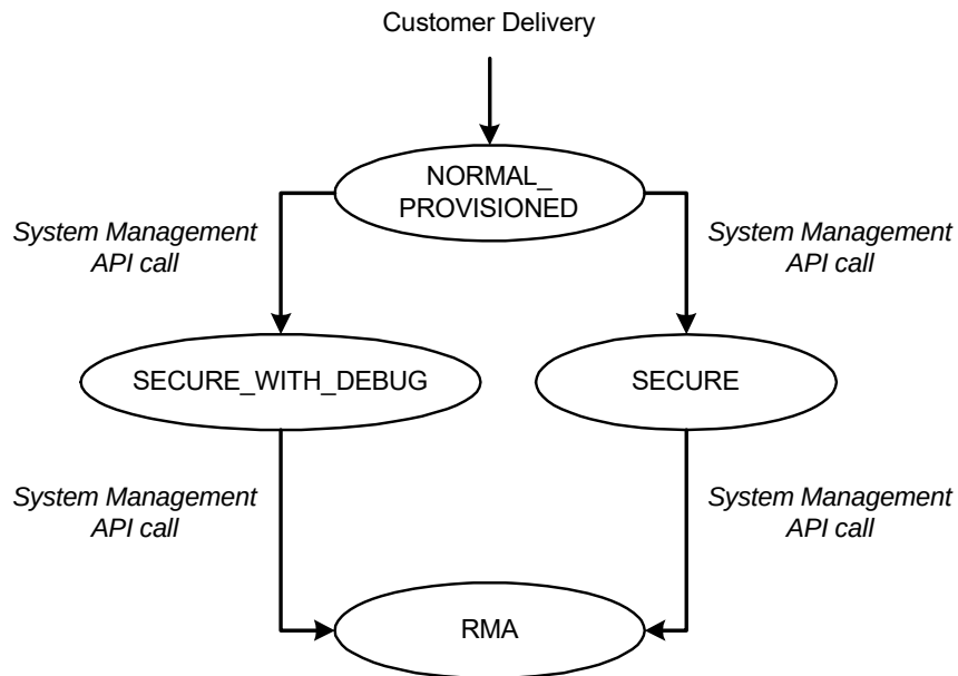
Figure 13-1. Traveo II Life Cycle Stage Transitions
