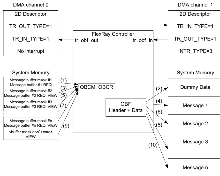
Figure 30-25. DMA Channel Configuration for Output Buffer Access (OBCM and OBCR)
