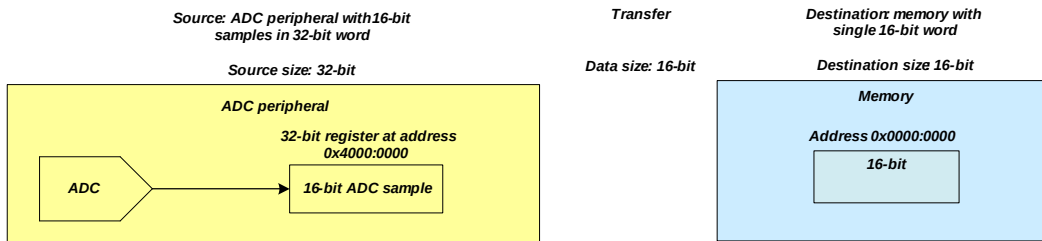
Figure 7-7. Single Transfer
