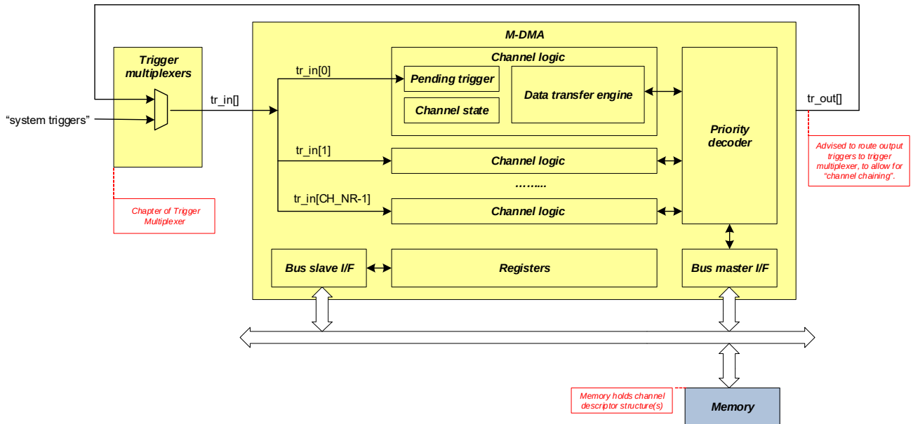
Figure 7-14. M-DMA Controller Design
