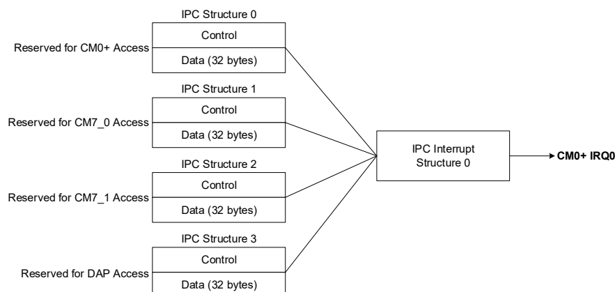
Figure 37-1. System Call Interface Using IPC
