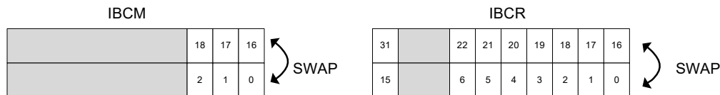
Figure 30-12. IBCM Register and IBCR Register Bit Swapping
