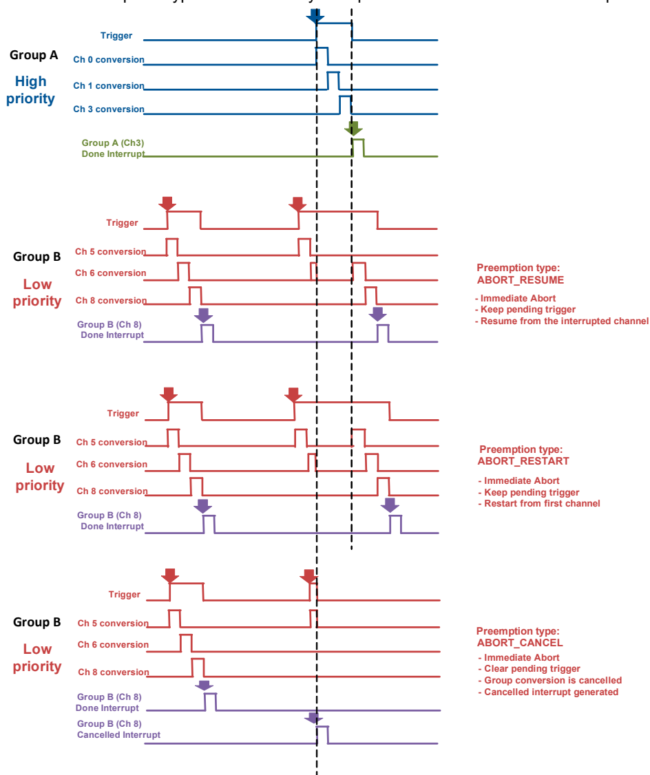
Figure 35-9. Preemption Types: A Low Priority Group B Behavior with Different Preemption Types
