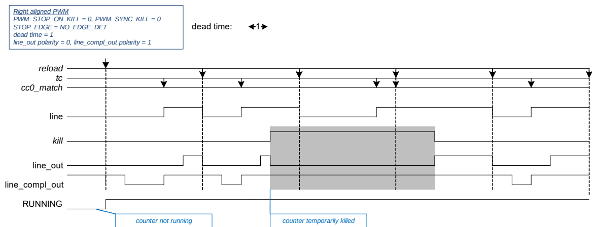
Figure 25-62. Dead Time and Kill
