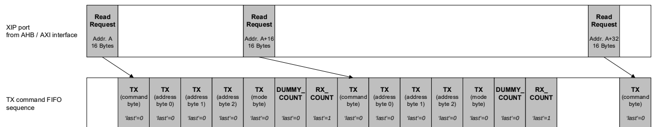
Figure 32-3. Read Sequence with Continuous Merging Disabled
