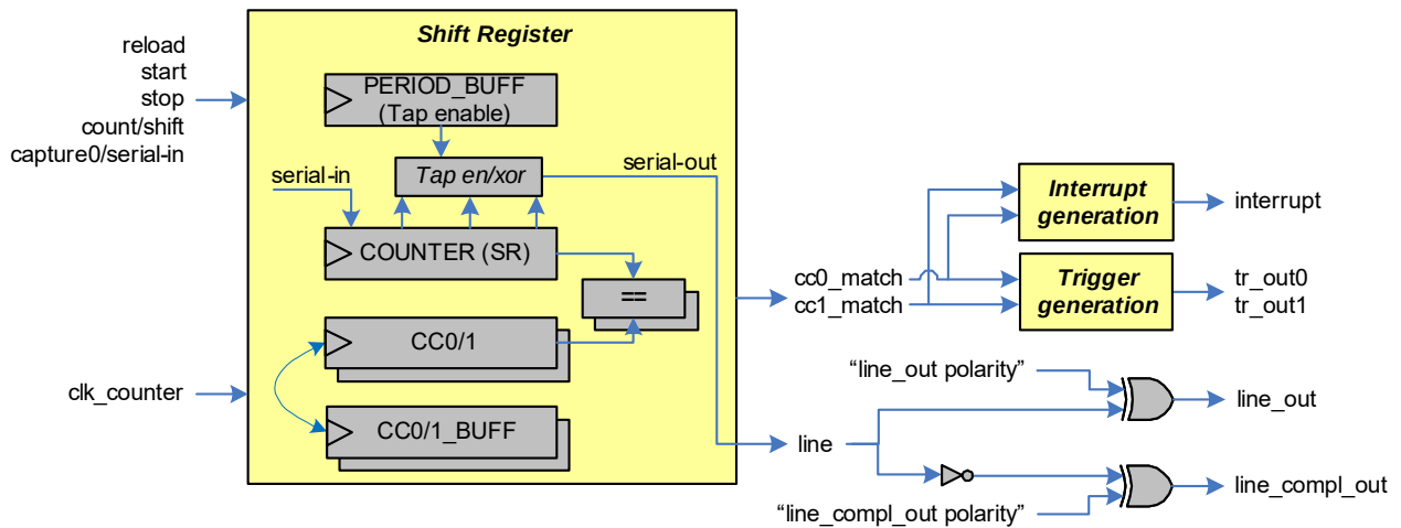
Figure 25-65. SR Function Diagram
