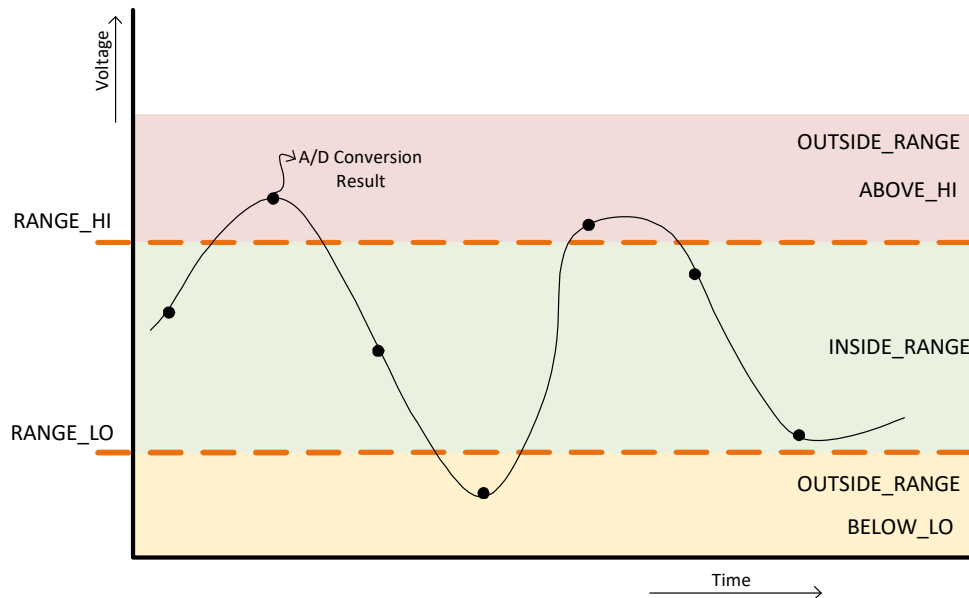
Figure 35-6. Range Detection, Threshold, and Events
