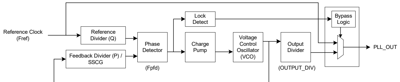
Figure 18-3. PLL with SSCG and Fractional Operation
