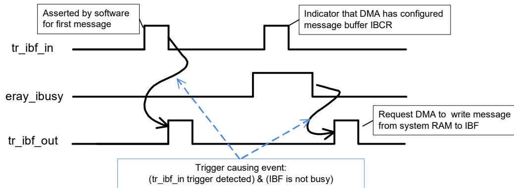
Figure 30-23. Trigger Interface Operation for IBF
