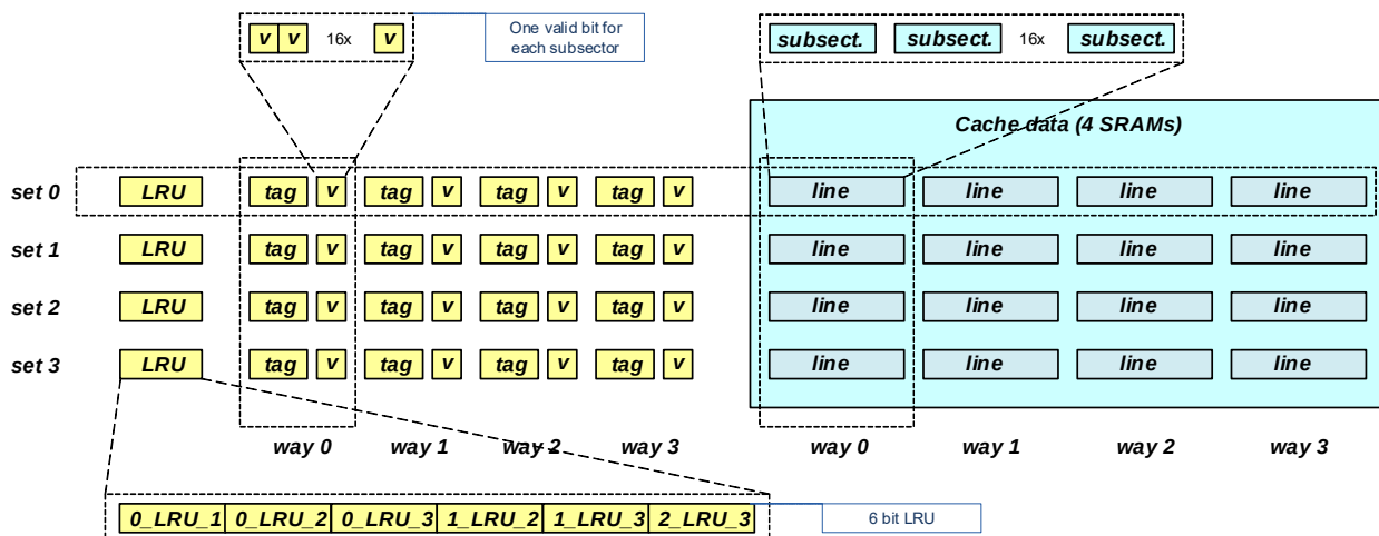
Figure 32-24. Cache Organization
