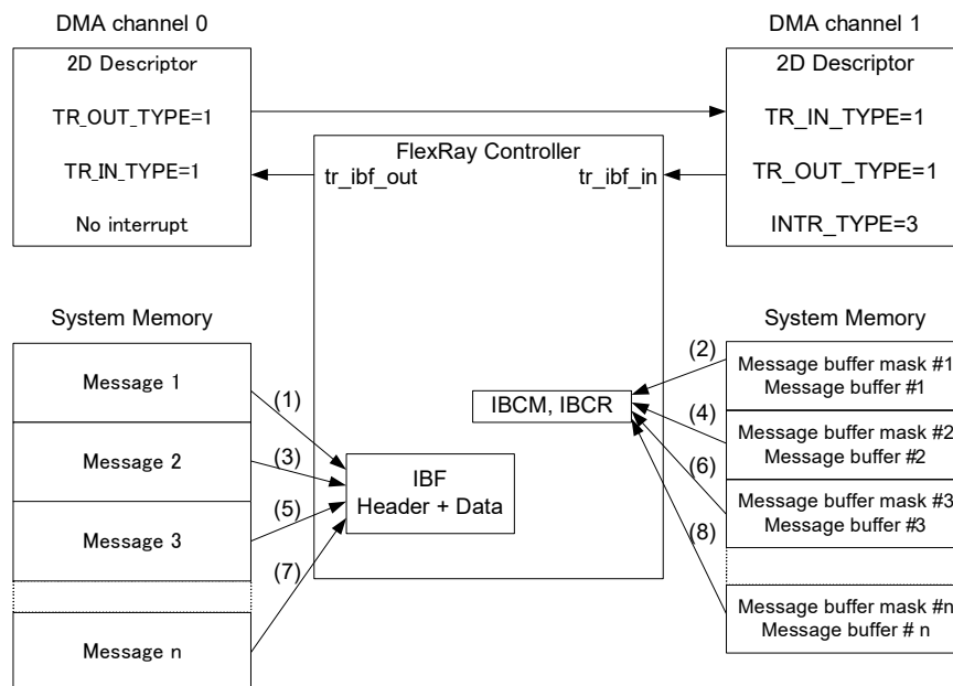
Figure 30-22. DMA Channel Configuration for Input Buffer Access (IBCM and IBCR)
