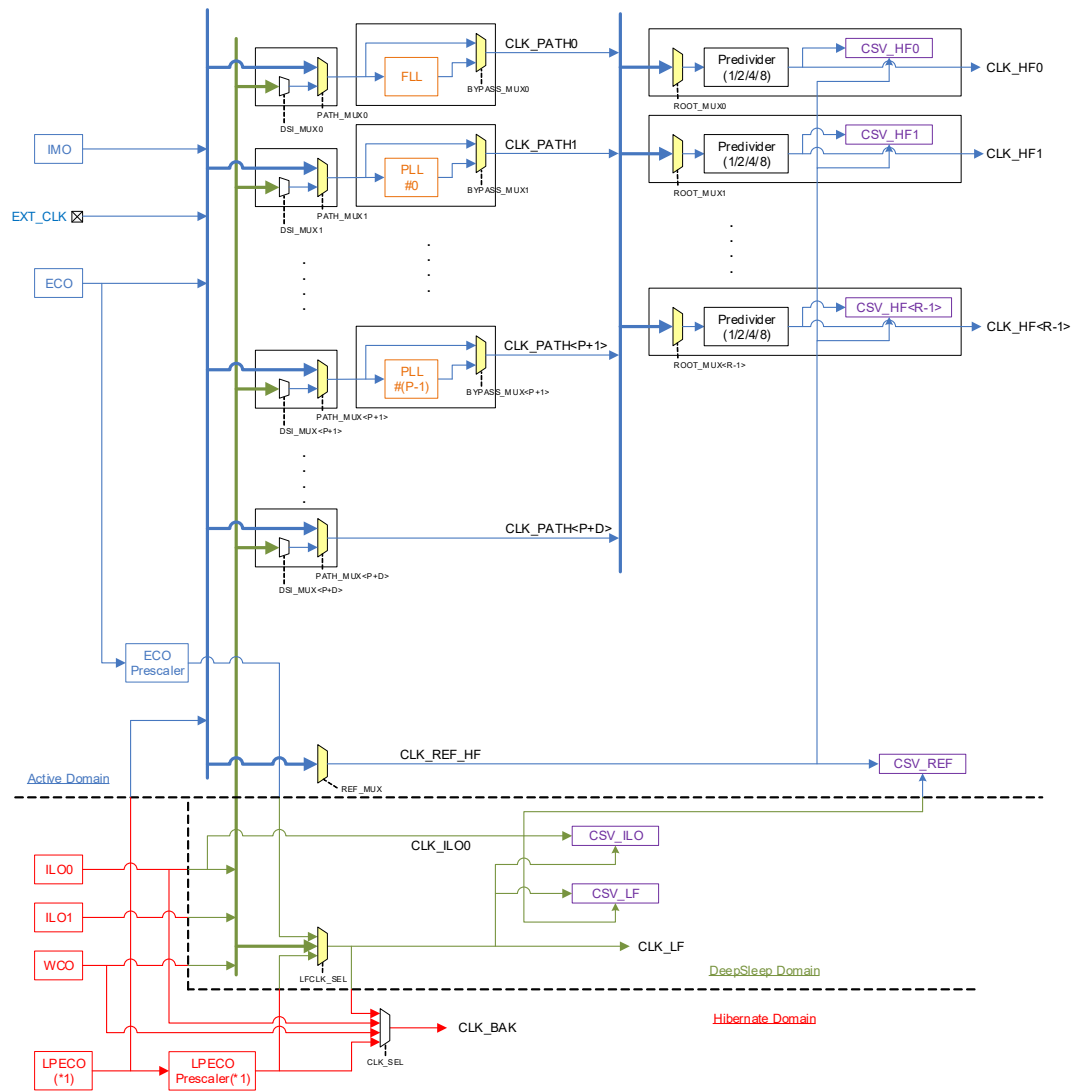
Figure 18-11. CSV Diagram
