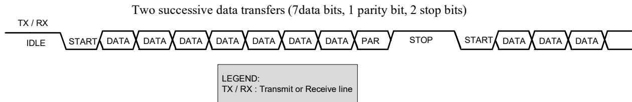
Figure 23-20. UART, Standard Protocol Example
