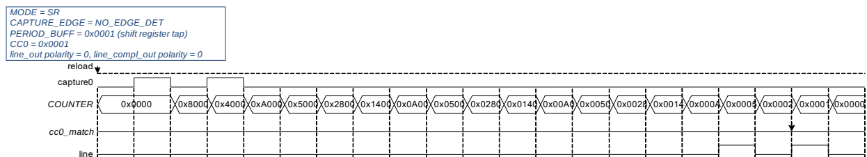
Figure 25-66. SR Shift with PERIOD_BUFF = 0x0001
