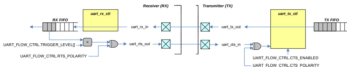
Figure 23-26. UART Flow Control Connection
