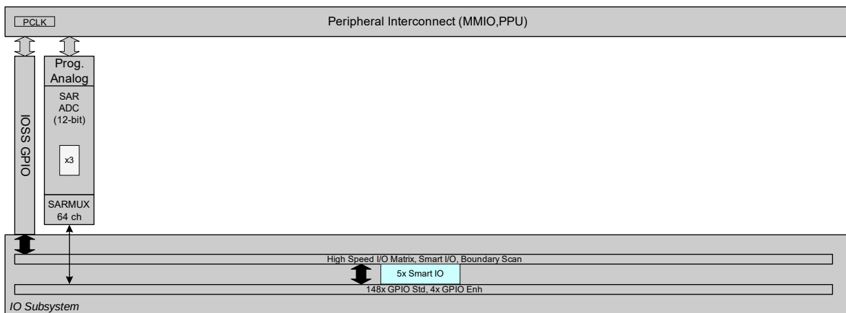
Analog System Block Diagram
