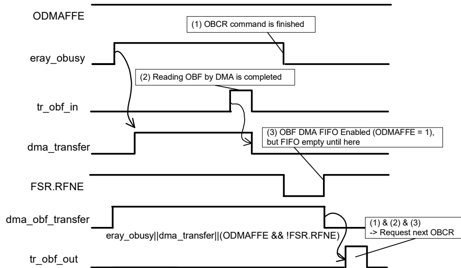
Figure 30-29. Case 4: Receive FIFO is Empty after OBCR
