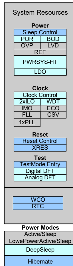
System-Wide Resources Block Diagram
