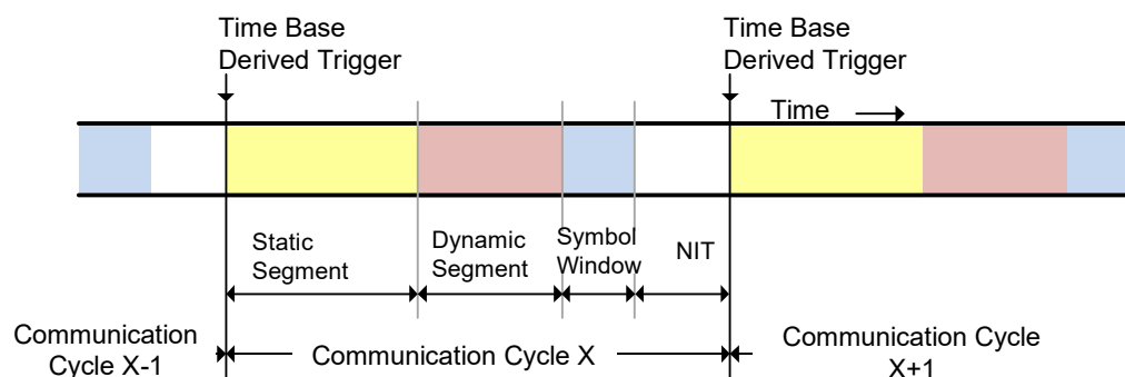
Figure 30-2. Communication Cycle Structure
