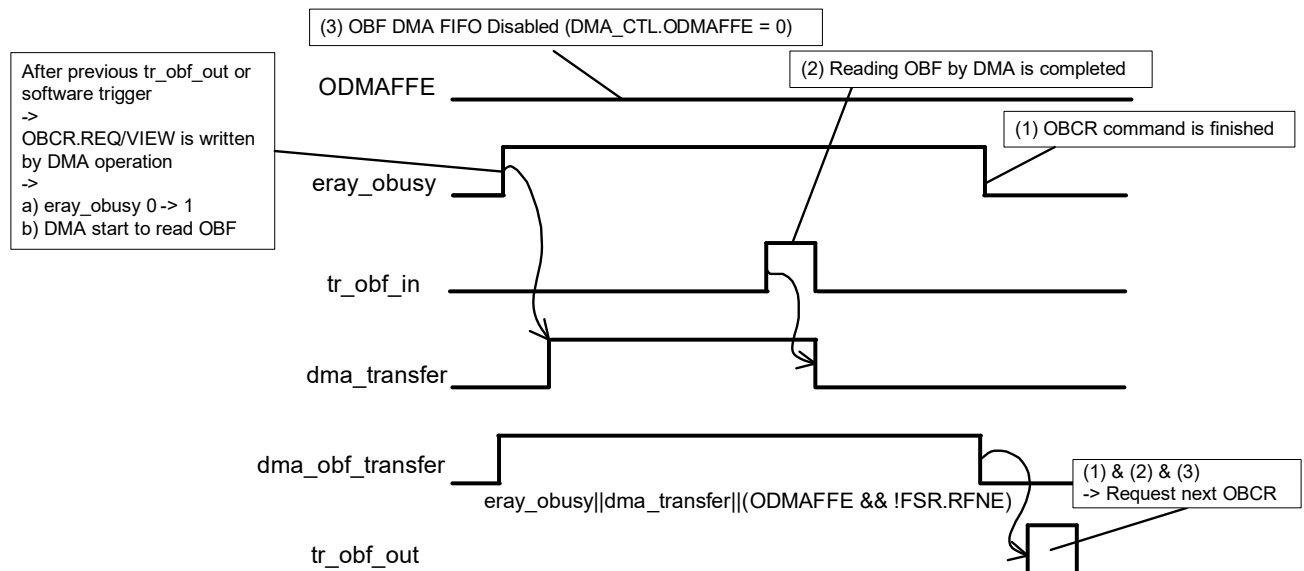
Figure 30-27. Case 2: Message Buffer RAM to OBF Transfer Takes Longer than DMA Transfer
