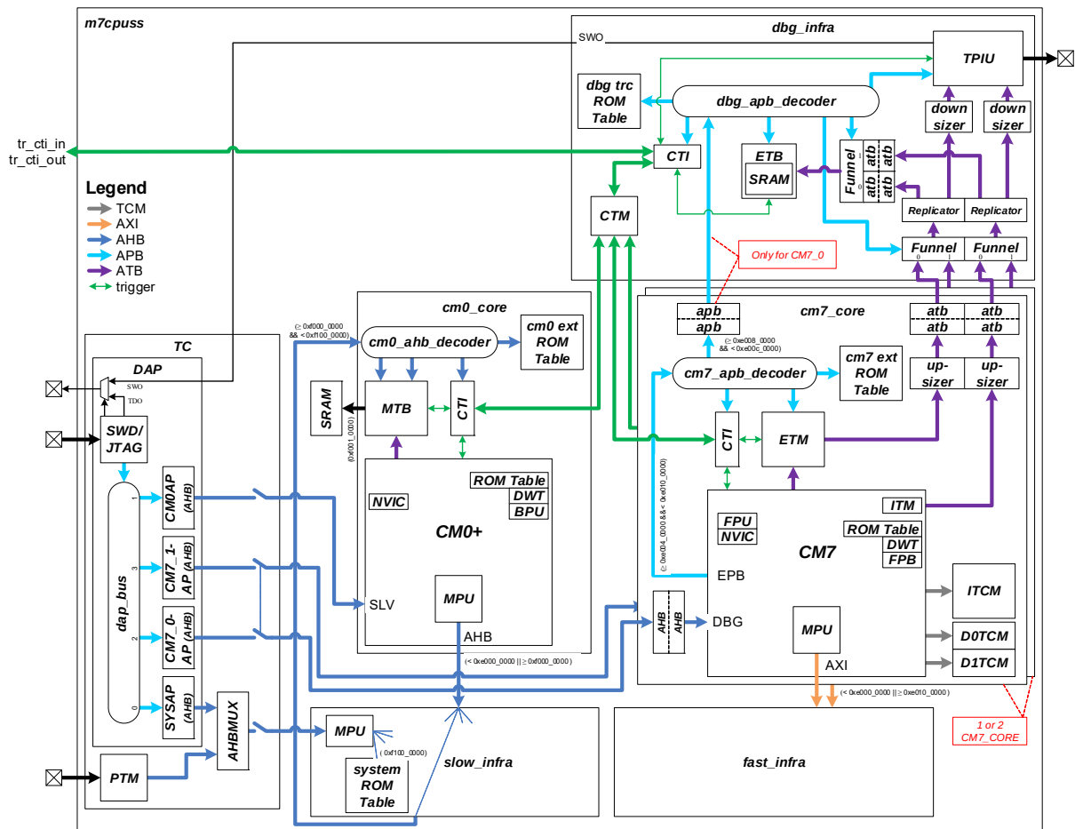
Program and Debug Architecture
