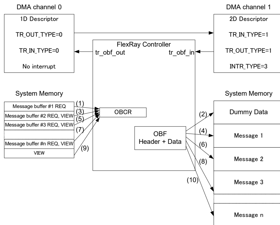
Figure 30-24. DMA Channel Configuration for Output Buffer Access (OBCR only)
