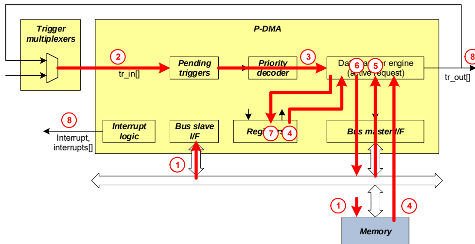
Figure 7-6. P-DMA Controller Flow
