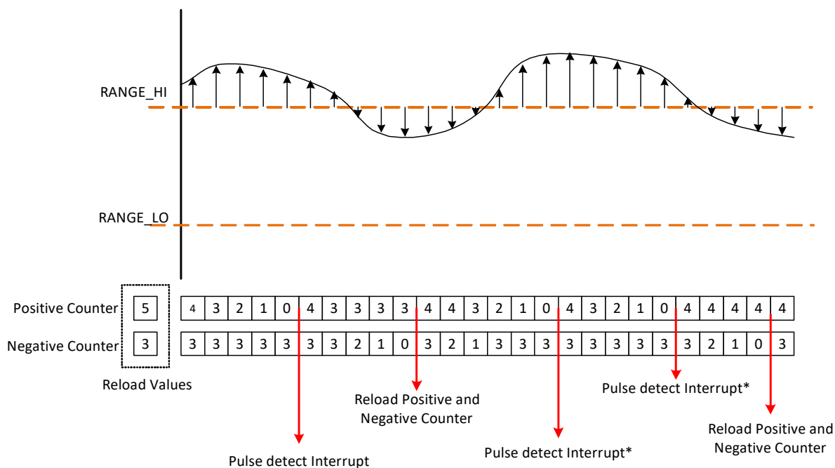
Figure 35-7. Pulse Detection
