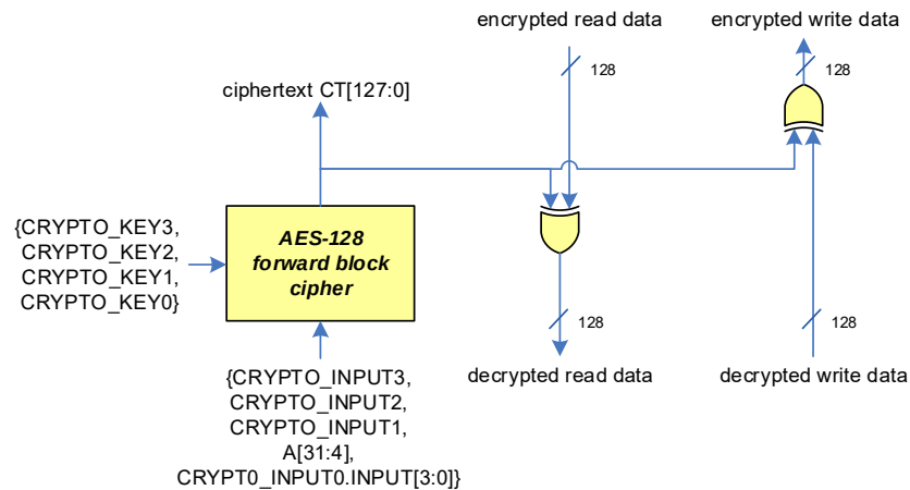
Figure 32-26. Cryptography in XIP Mode
