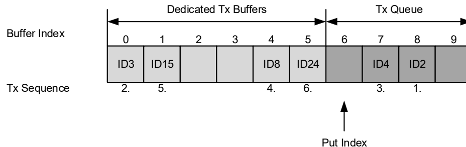
Figure 24-13. Example of Mixed Configuration Dedicated TX Buffers/TX Queue
