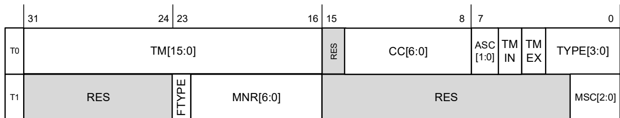
Figure 24-23. Trigger Memory Element
