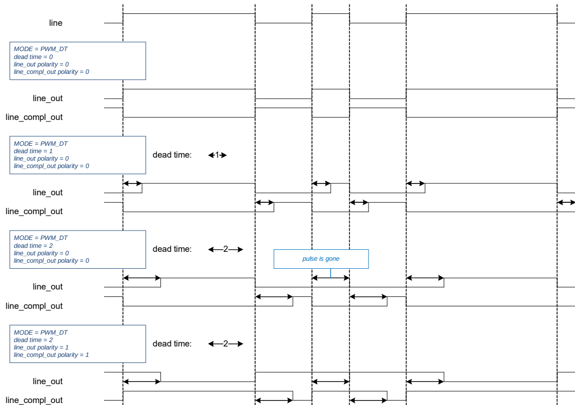
Figure 25-61. Dead-time Timing
