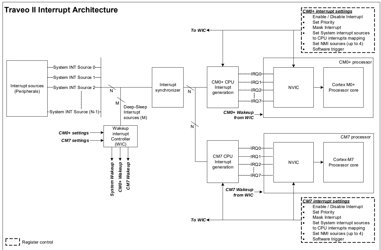
Figure 12-1. Traveo II Interrupts Block Diagram
