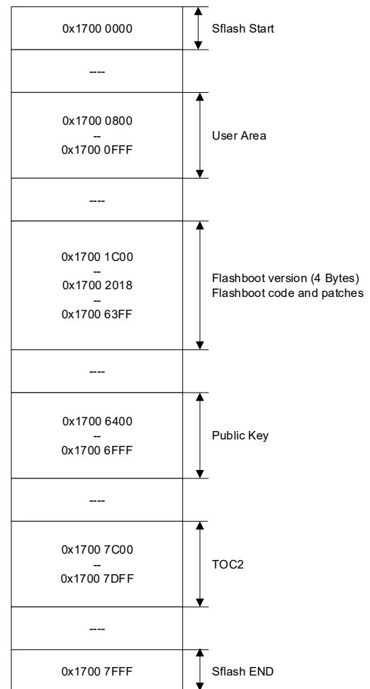
Figure 38-10. SFlash Address Mapping
