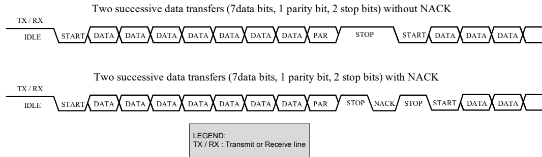
Figure 23-35. SmartCard Example
