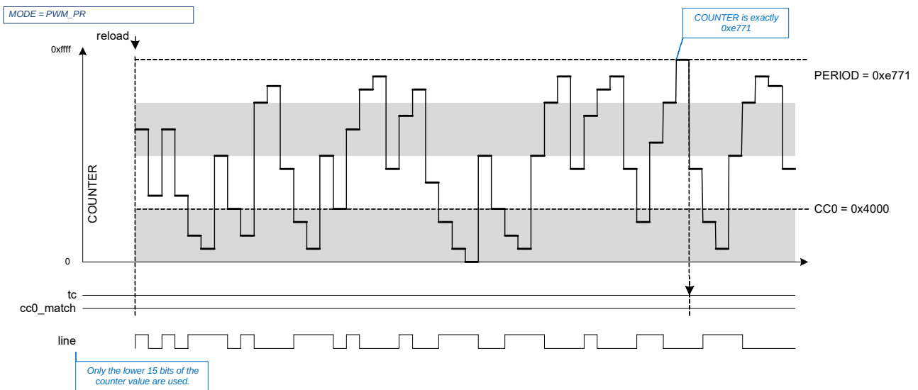
Figure 25-64. PWM_PR Output
