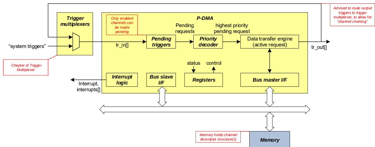
Figure 7-5. P-DMA Controller Design
