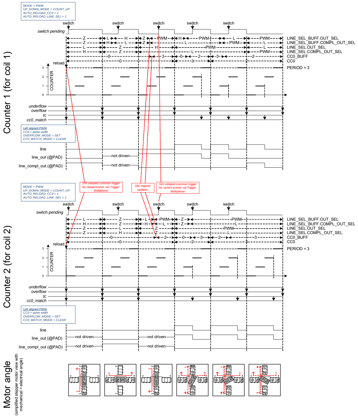
Figure 25-59. PWM Output for Stepper Motor
