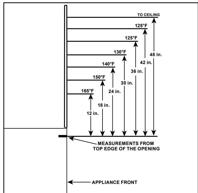
Figure 3.3. Wall Surface Temperatures Above Appliance (MEZZO36-B/MEZZO36ST-B/MEZZO48-B/MEZZO48ST-B)
