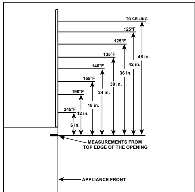
Figure 3.4. Wall Surface Temperatures Above Appliance (MEZZO60-B/MEZZO60ST-B/MEZZO72-B/MEZZO72ST-B)
