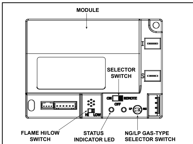
Figure 3.8 Control Module
